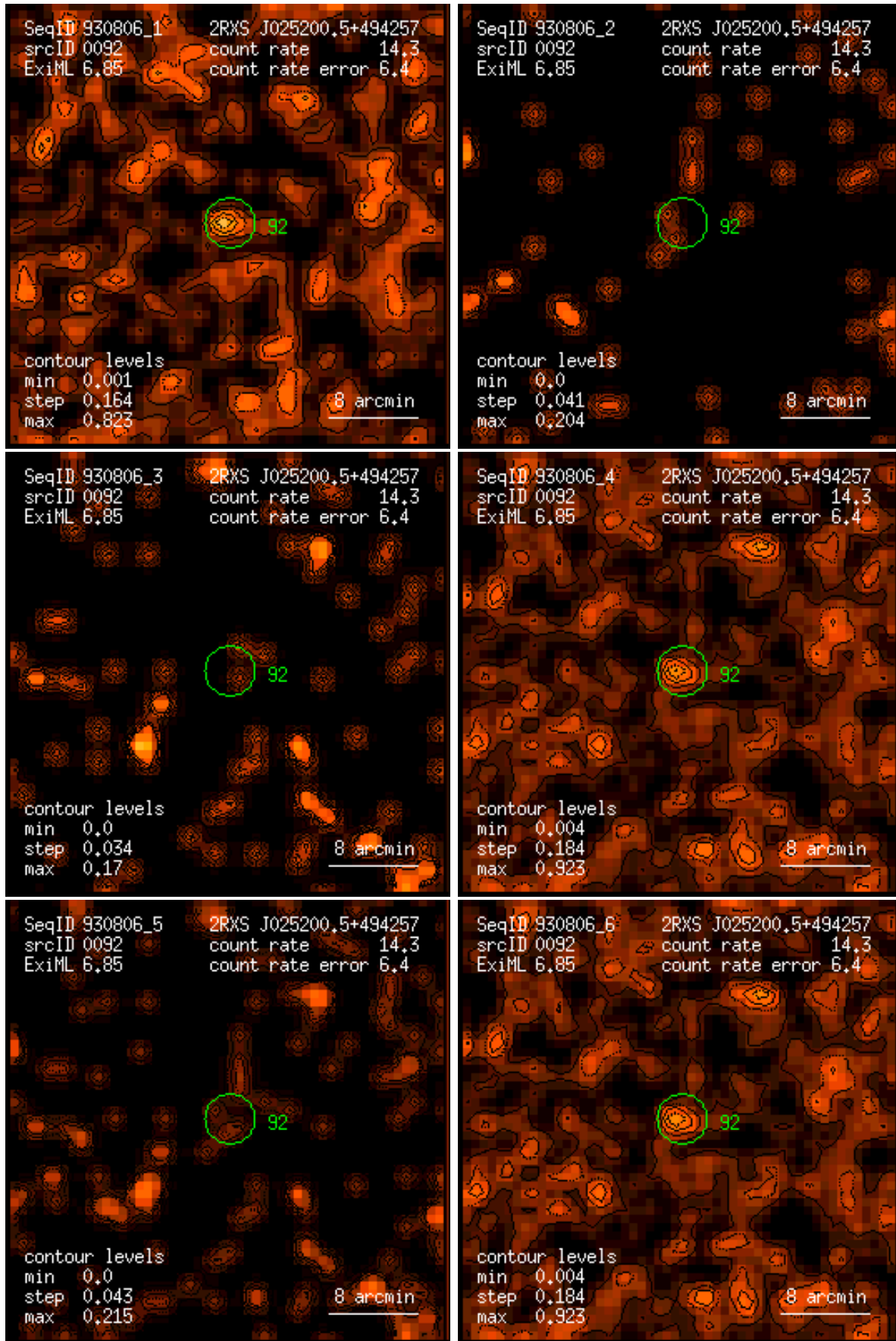
Figure 92: RASS 930806: detection 0092: band rate images, Gaussian filter: (1) PSPC channels 11 – 41, (2) 52 – 90, (3) 91 – 201, (4) 11 – 235, (5) 52 – 201, (6) 11 – 201. Broad band rates in counts/ks. Band rate contour levels in counts/ks/arcmin 2 .
