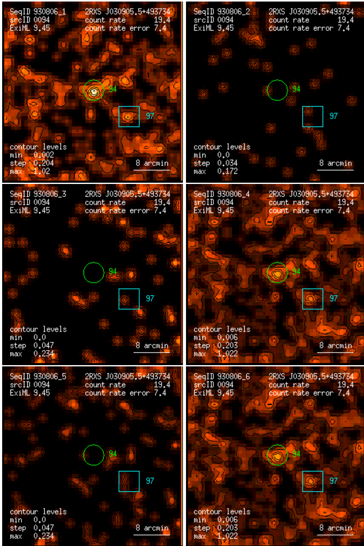
Figure 94: RASS 930806: detection 0094: band rate images, Gaussian filter: (1) PSPC channels 11 – 41, (2) 52 – 90, (3) 91 – 201, (4) 11 – 235, (5) 52 – 201, (6) 11 – 201. Broad band rates in counts/ks. Band rate contour levels in counts/ks/arcmin 2 .
