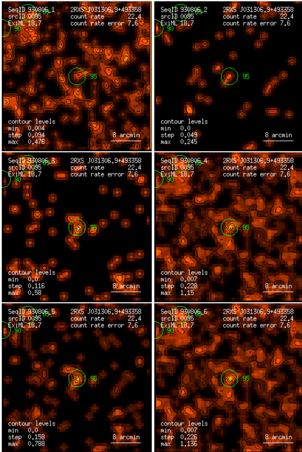
Figure 95: RASS 930806: detection 0095: band rate images, Gaussian filter: (1) PSPC channels 11 – 41, (2) 52 – 90, (3) 91 – 201, (4) 11 – 235, (5) 52 – 201, (6) 11 – 201. Broad band rates in counts/ks. Band rate contour levels in counts/ks/arcmin 2 .
