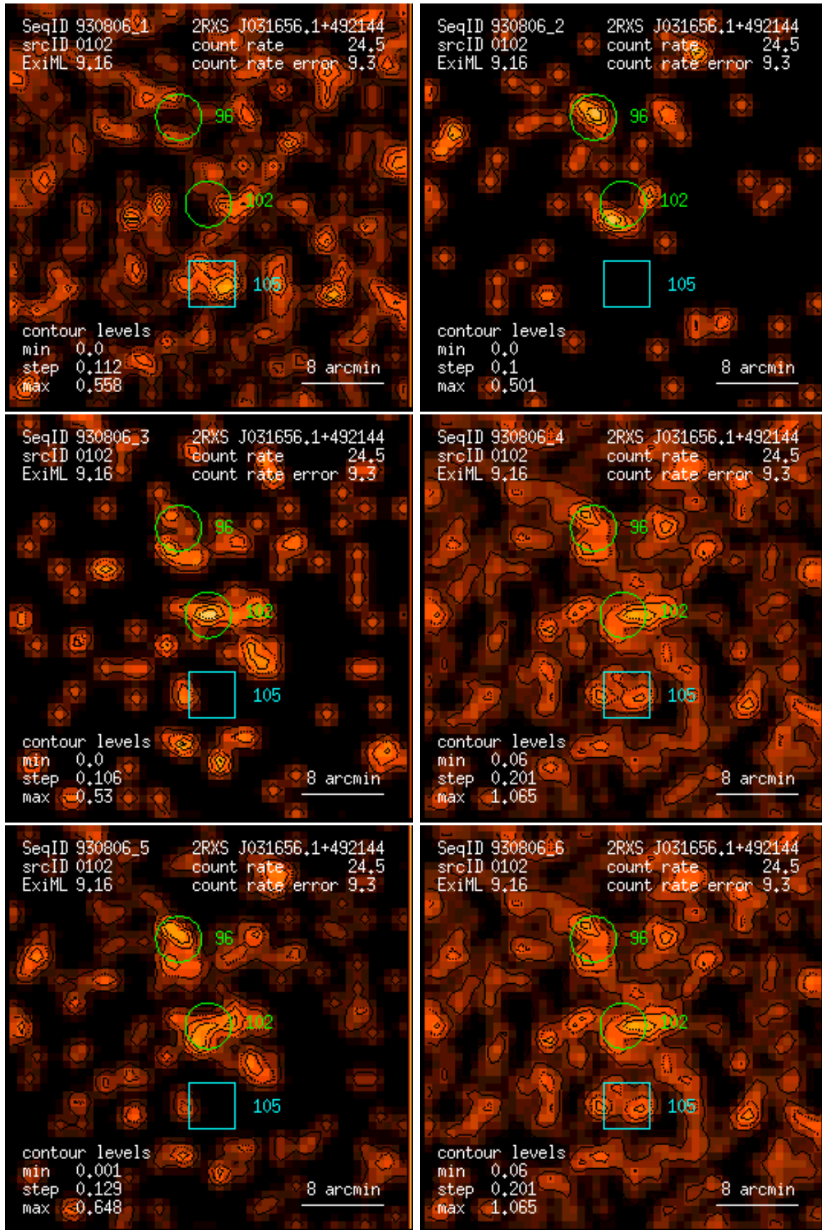
Figure 102: RASS 930806: detection 0102: band rate images, Gaussian filter: (1) PSPC channels 11 – 41, (2) 52 – 90, (3) 91 – 201, (4) 11 – 235, (5) 52 – 201, (6) 11 – 201. Broad band rates in counts/ks. Band rate contour levels in counts/ks/arcmin 2 .
