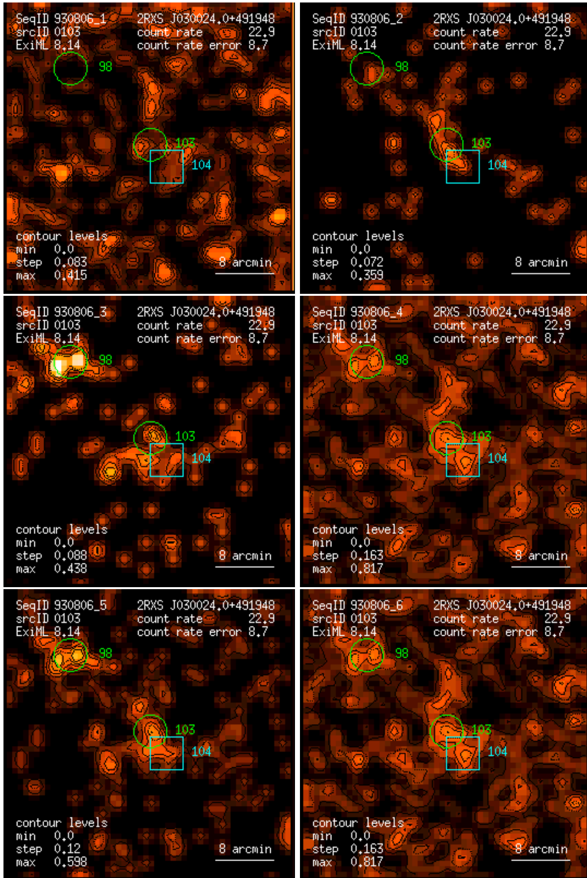
Figure 103: RASS 930806: detection 0103: band rate images, Gaussian filter: (1) PSPC channels 11 – 41, (2) 52 – 90, (3) 91 – 201, (4) 11 – 235, (5) 52 – 201, (6) 11 – 201. Broad band rates in counts/ks. Band rate contour levels in counts/ks/arcmin 2 .
