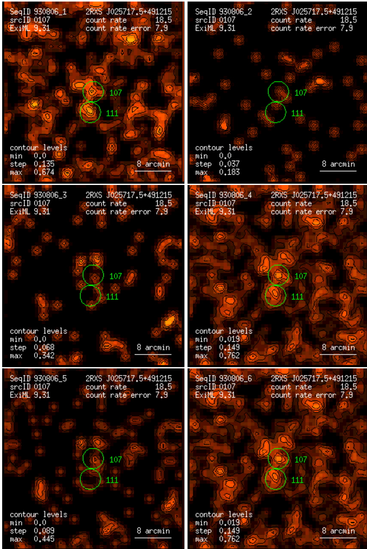
Figure 107: RASS 930806: detection 0107: band rate images, Gaussian filter: (1) PSPC channels 11 – 41, (2) 52 – 90, (3) 91 – 201, (4) 11 – 235, (5) 52 – 201, (6) 11 – 201. Broad band rates in counts/ks. Band rate contour levels in counts/ks/arcmin 2 .
