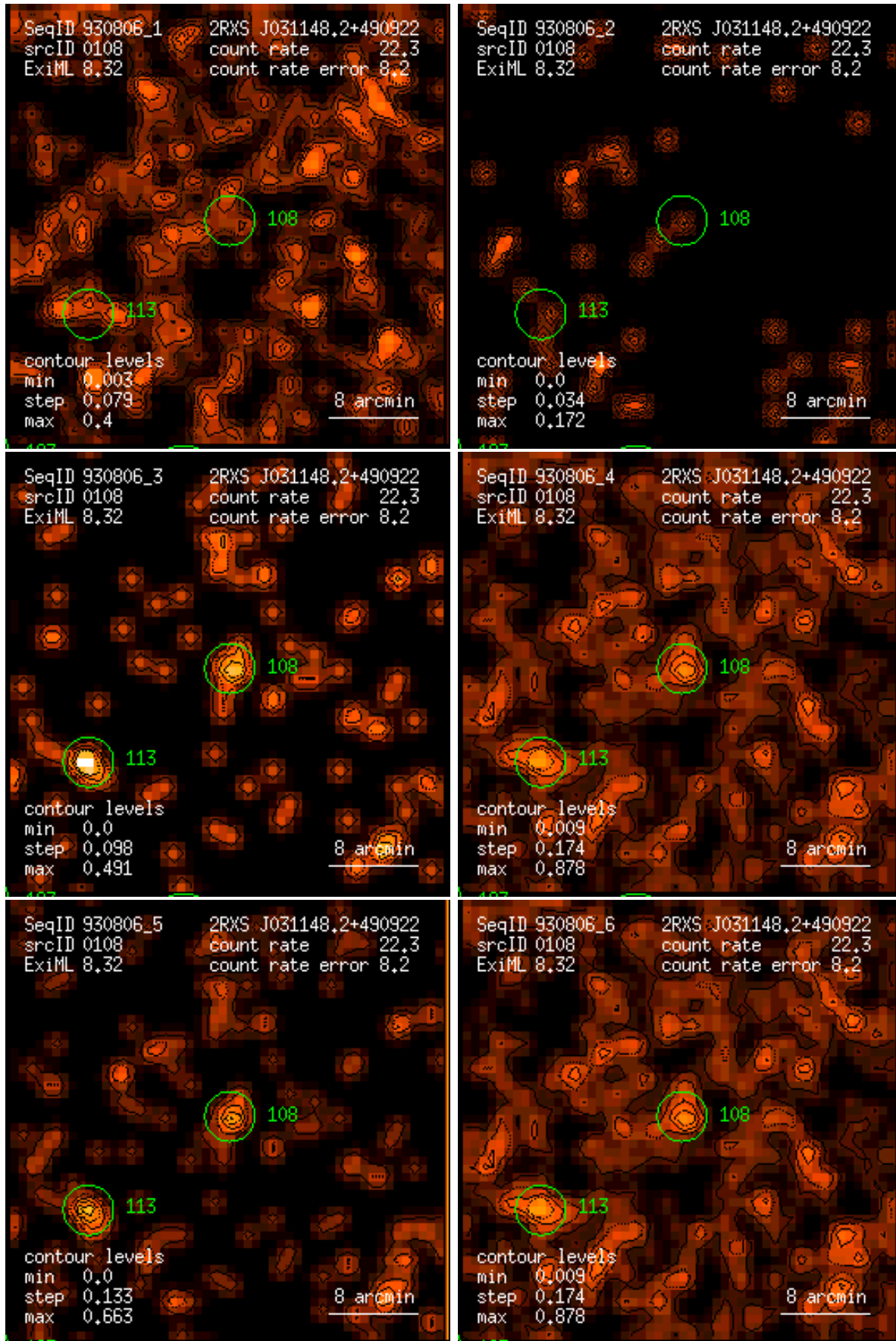
Figure 108: RASS 930806: detection 0108: band rate images, Gaussian filter: (1) PSPC channels 11 – 41, (2) 52 – 90, (3) 91 – 201, (4) 11 – 235, (5) 52 – 201, (6) 11 – 201. Broad band rates in counts/ks. Band rate contour levels in counts/ks/arcmin 2 .
