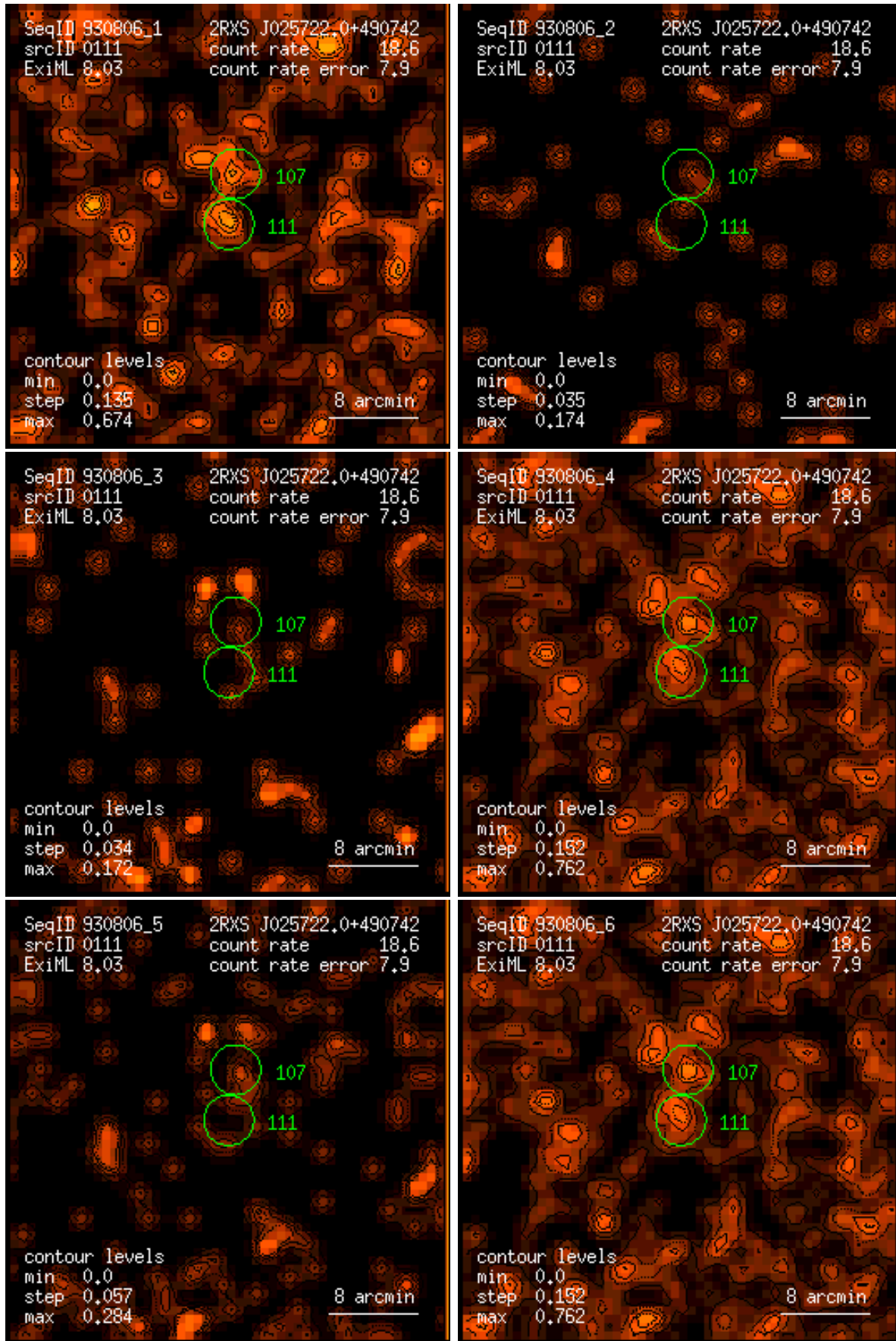
Figure 111: RASS 930806: detection 0111: band rate images, Gaussian filter: (1) PSPC channels 11 – 41, (2) 52 – 90, (3) 91 – 201, (4) 11 – 235, (5) 52 – 201, (6) 11 – 201. Broad band rates in counts/ks. Band rate contour levels in counts/ks/arcmin 2 .
