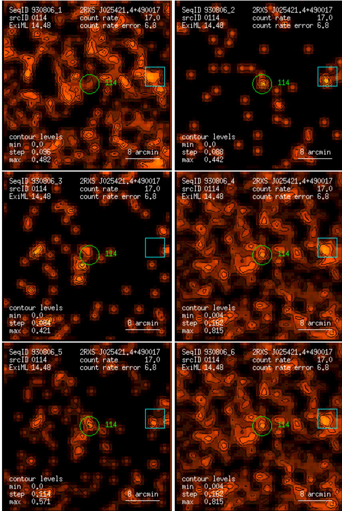
Figure 114: RASS 930806: detection 0114: band rate images, Gaussian filter: (1) PSPC channels 11 – 41, (2) 52 – 90, (3) 91 – 201, (4) 11 – 235, (5) 52 – 201, (6) 11 – 201. Broad band rates in counts/ks. Band rate contour levels in counts/ks/arcmin 2 .
