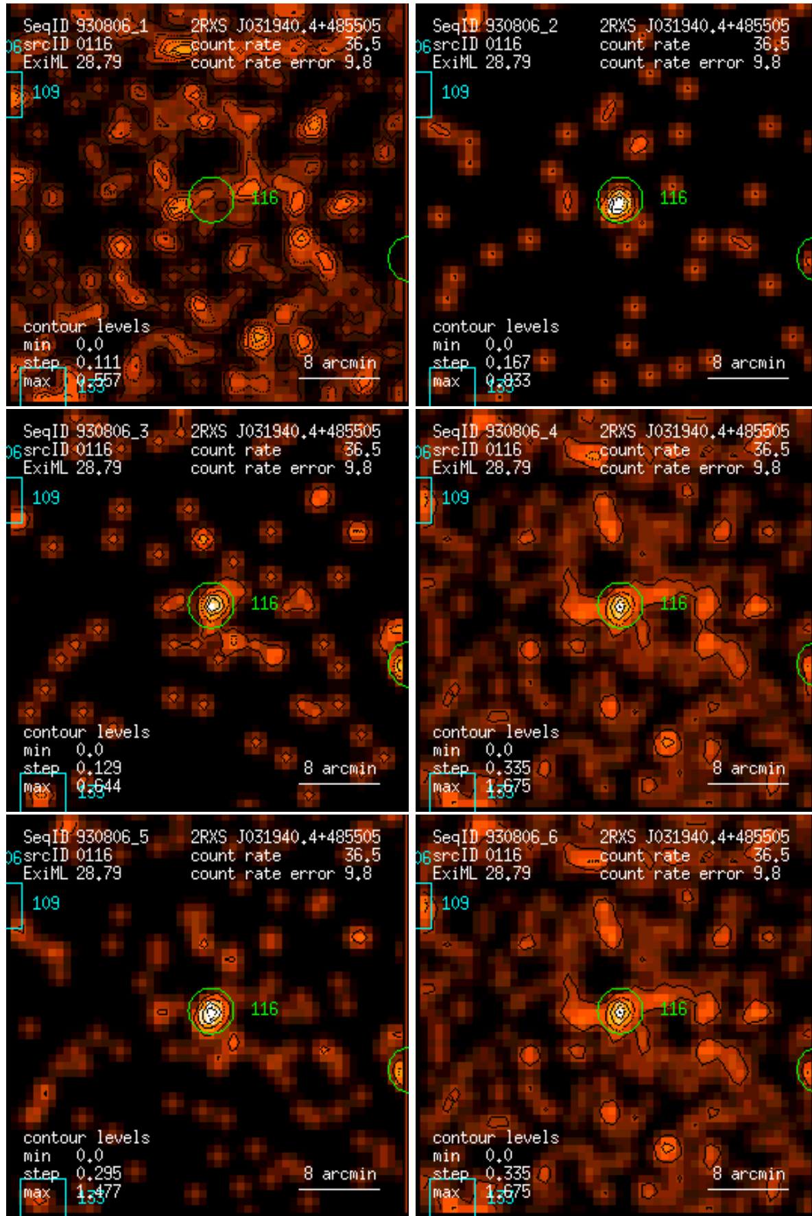
Figure 116: RASS 930806: detection 0116: band rate images, Gaussian filter: (1) PSPC channels 11 – 41, (2) 52 – 90, (3) 91 – 201, (4) 11 – 235, (5) 52 – 201, (6) 11 – 201. Broad band rates in counts/ks. Band rate contour levels in counts/ks/arcmin 2 .
