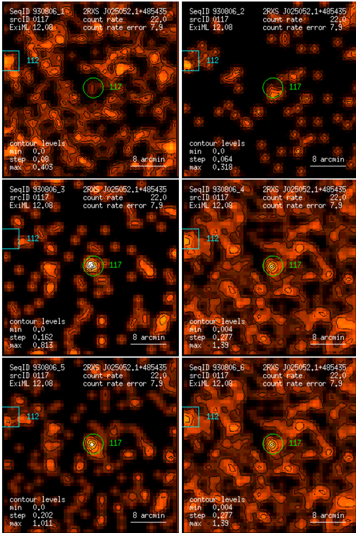
Figure 117: RASS 930806: detection 0117: band rate images, Gaussian filter: (1) PSPC channels 11 – 41, (2) 52 – 90, (3) 91 – 201, (4) 11 – 235, (5) 52 – 201, (6) 11 – 201. Broad band rates in counts/ks. Band rate contour levels in counts/ks/arcmin 2 .
