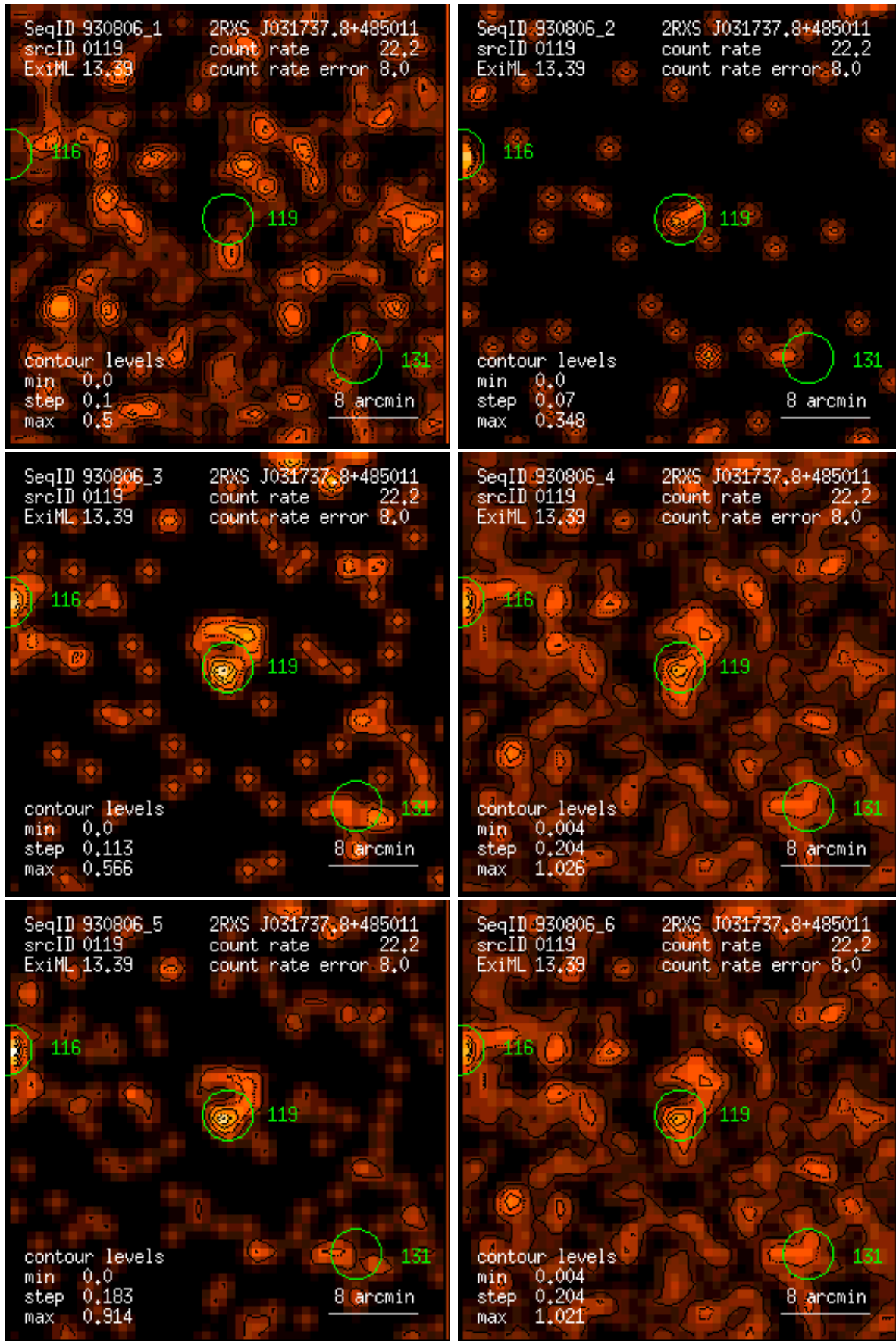
Figure 119: RASS 930806: detection 0119: band rate images, Gaussian filter: (1) PSPC channels 11 – 41, (2) 52 – 90, (3) 91 – 201, (4) 11 – 235, (5) 52 – 201, (6) 11 – 201. Broad band rates in counts/ks. Band rate contour levels in counts/ks/arcmin 2 .
