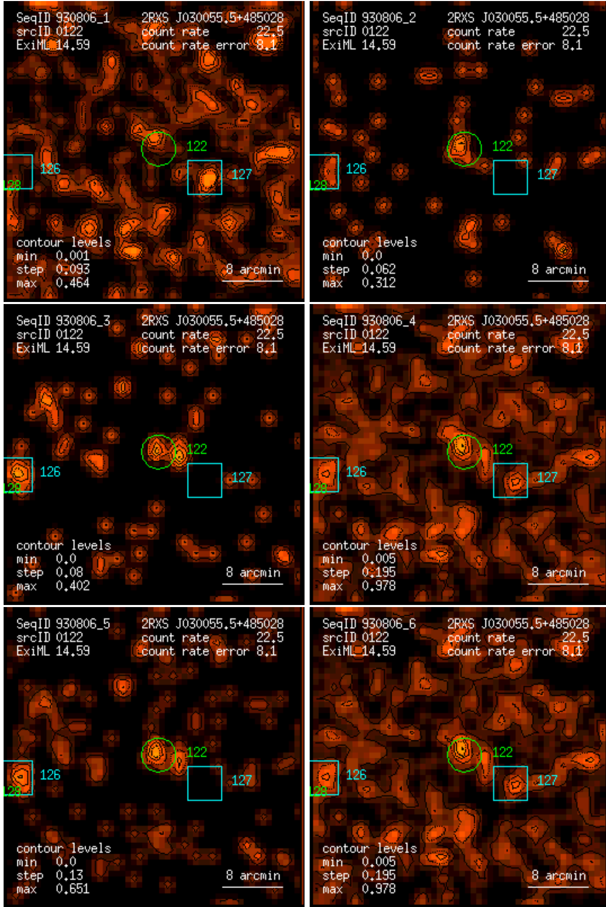
Figure 122: RASS 930806: detection 0122: band rate images, Gaussian filter: (1) PSPC channels 11 – 41, (2) 52 – 90, (3) 91 – 201, (4) 11 – 235, (5) 52 – 201, (6) 11 – 201. Broad band rates in counts/ks. Band rate contour levels in counts/ks/arcmin 2 .
