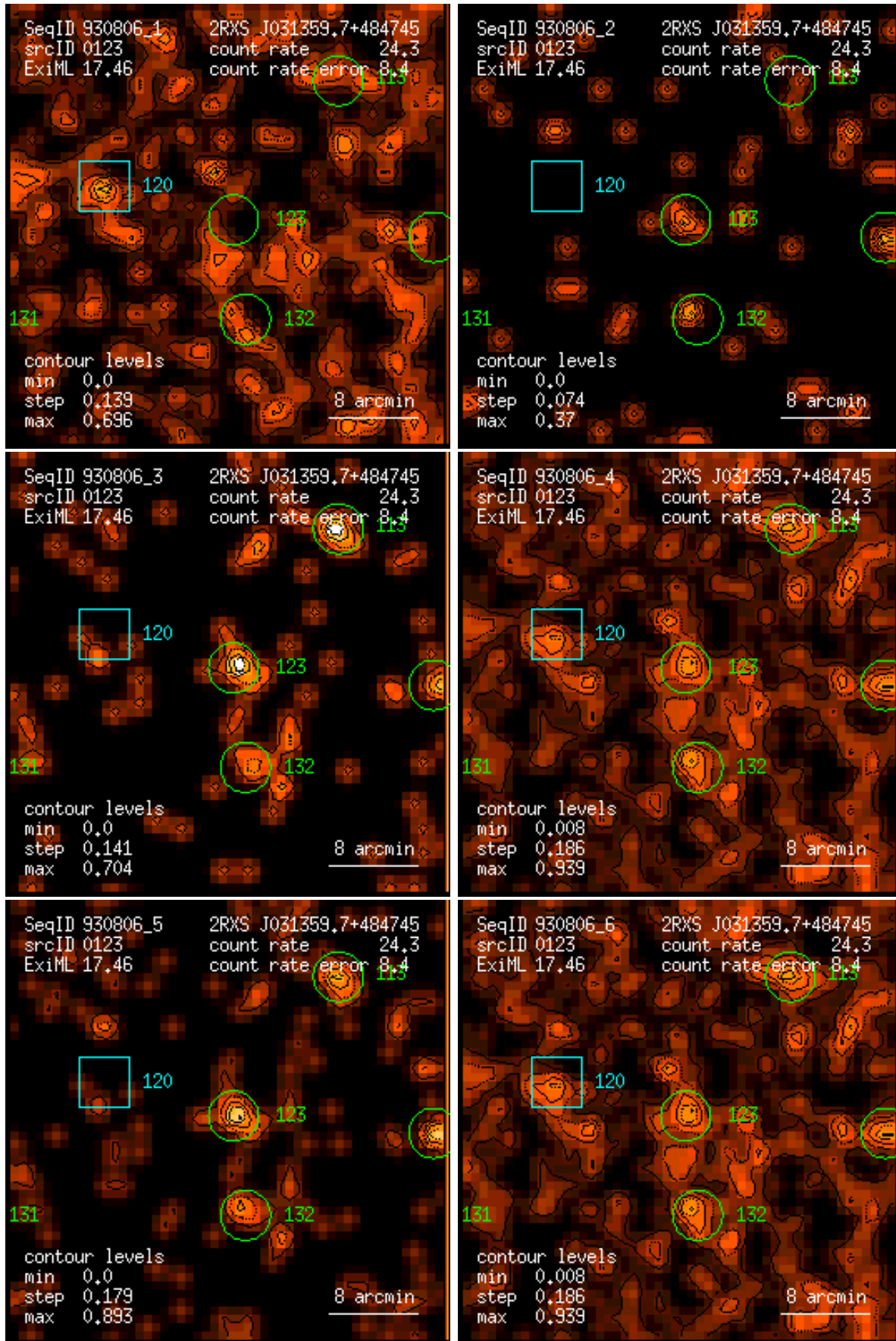
Figure 123: RASS 930806: detection 0123: band rate images, Gaussian filter: (1) PSPC channels 11 – 41, (2) 52 – 90, (3) 91 – 201, (4) 11 – 235, (5) 52 – 201, (6) 11 – 201. Broad band rates in counts/ks. Band rate contour levels in counts/ks/arcmin 2 .
