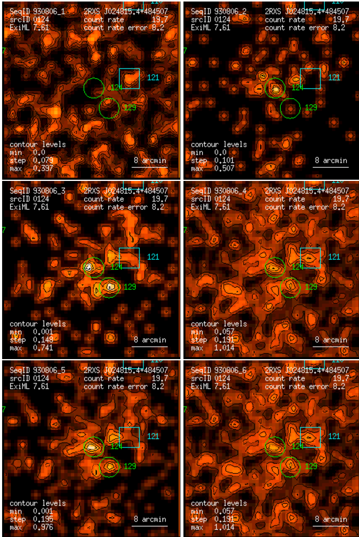
Figure 124: RASS 930806: detection 0124: band rate images, Gaussian filter: (1) PSPC channels 11 – 41, (2) 52 – 90, (3) 91 – 201, (4) 11 – 235, (5) 52 – 201, (6) 11 – 201. Broad band rates in counts/ks. Band rate contour levels in counts/ks/arcmin 2 .
