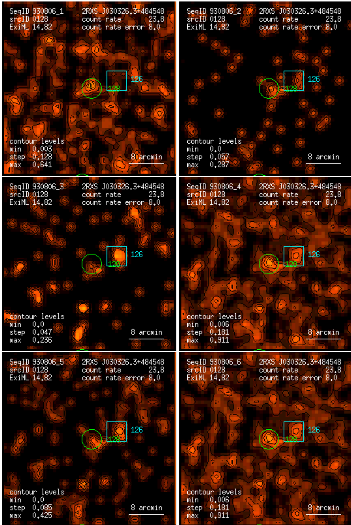
Figure 128: RASS 930806: detection 0128: band rate images, Gaussian filter: (1) PSPC channels 11 – 41, (2) 52 – 90, (3) 91 – 201, (4) 11 – 235, (5) 52 – 201, (6) 11 – 201. Broad band rates in counts/ks. Band rate contour levels in counts/ks/arcmin 2 .
