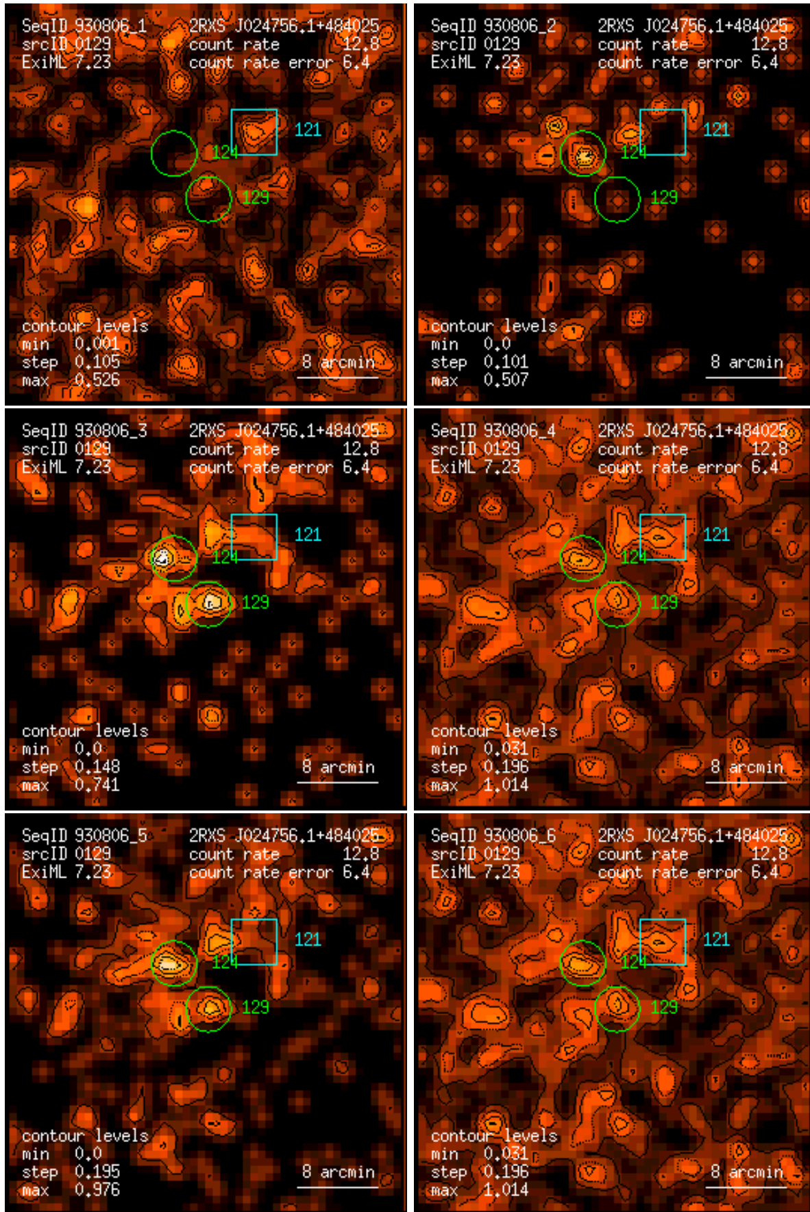
Figure 129: RASS 930806: detection 0129: band rate images, Gaussian filter: (1) PSPC channels 11 – 41, (2) 52 – 90, (3) 91 – 201, (4) 11 – 235, (5) 52 – 201, (6) 11 – 201. Broad band rates in counts/ks. Band rate contour levels in counts/ks/arcmin 2 .
