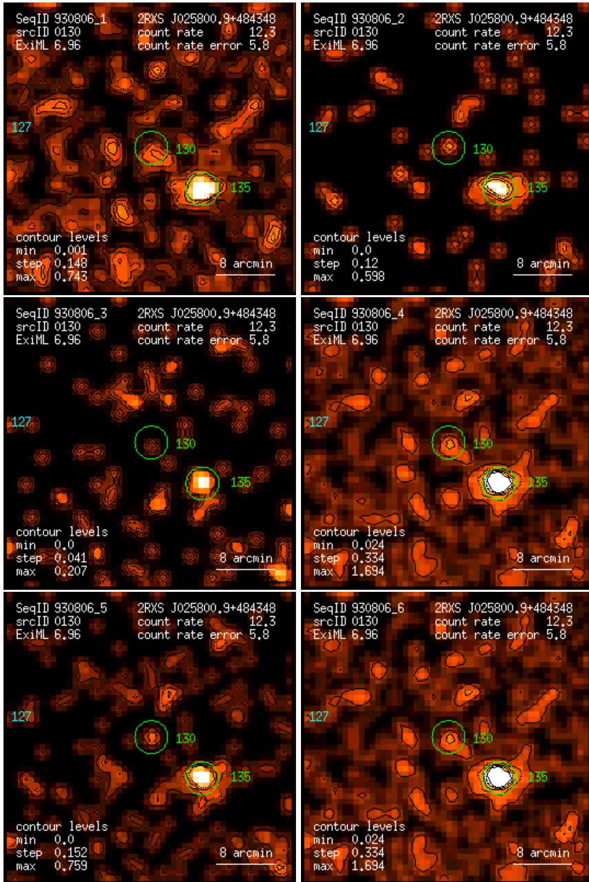
Figure 130: RASS 930806: detection 0130: band rate images, Gaussian filter: (1) PSPC channels 11 – 41, (2) 52 – 90, (3) 91 – 201, (4) 11 – 235, (5) 52 – 201, (6) 11 – 201. Broad band rates in counts/ks. Band rate contour levels in counts/ks/arcmin 2 .
