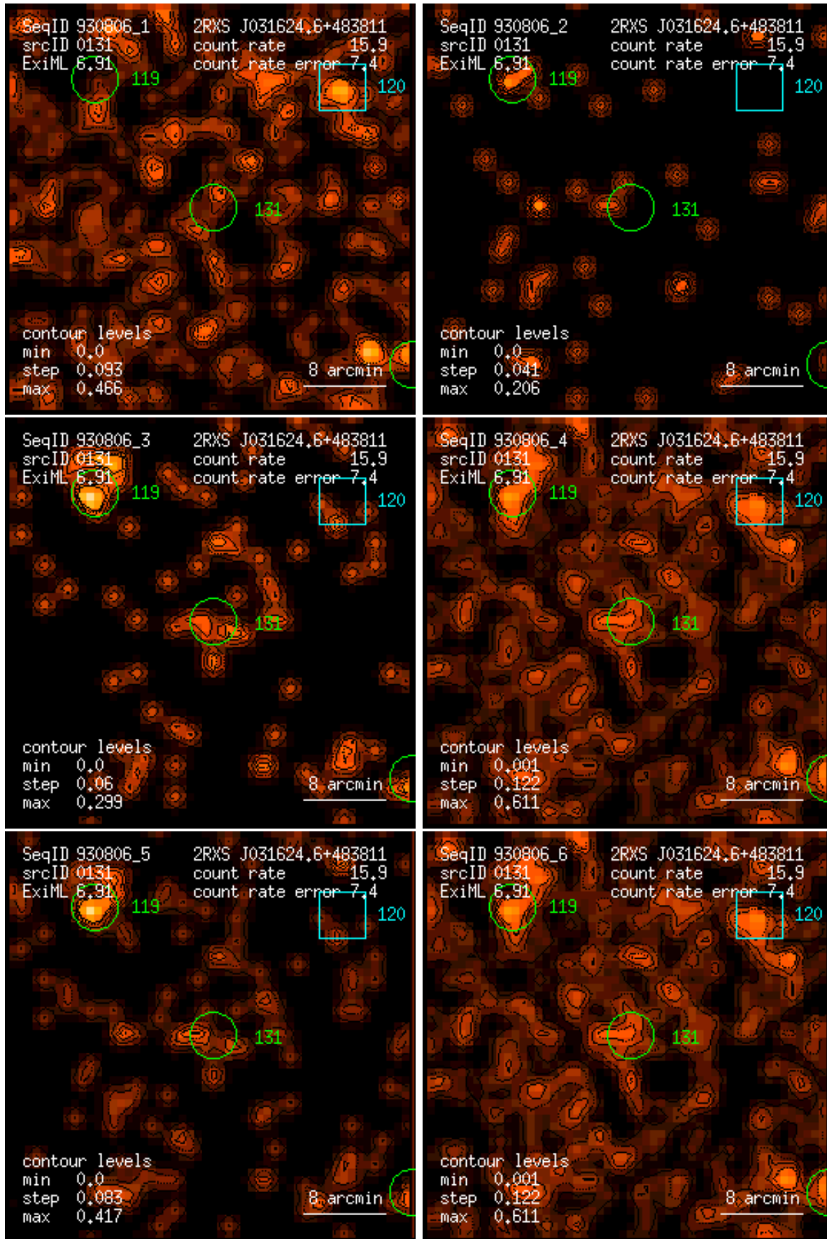
Figure 131: RASS 930806: detection 0131: band rate images, Gaussian filter: (1) PSPC channels 11 – 41, (2) 52 – 90, (3) 91 – 201, (4) 11 – 235, (5) 52 – 201, (6) 11 – 201. Broad band rates in counts/ks. Band rate contour levels in counts/ks/arcmin 2 .
