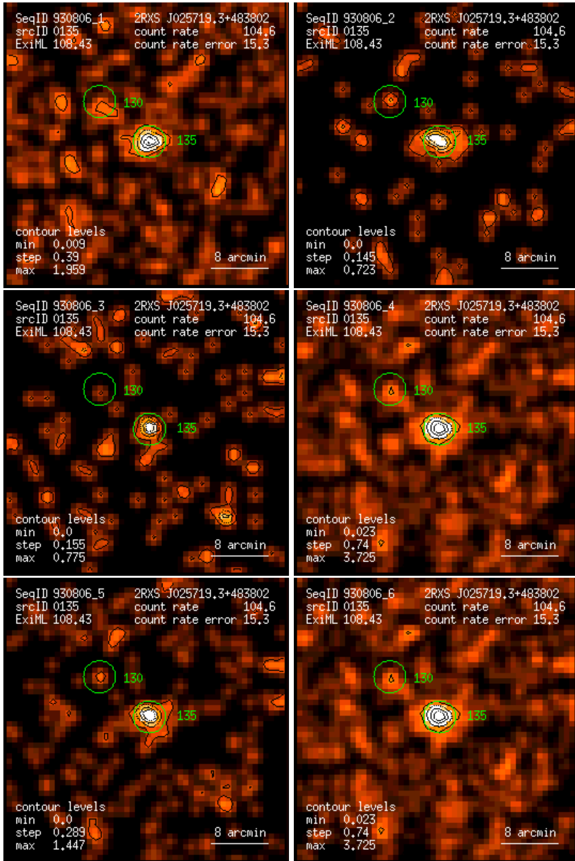
Figure 135: RASS 930806: detection 0135: band rate images, Gaussian filter: (1) PSPC channels 11 – 41, (2) 52 – 90, (3) 91 – 201, (4) 11 – 235, (5) 52 – 201, (6) 11 – 201. Broad band rates in counts/ks. Band rate contour levels in counts/ks/arcmin 2 .
