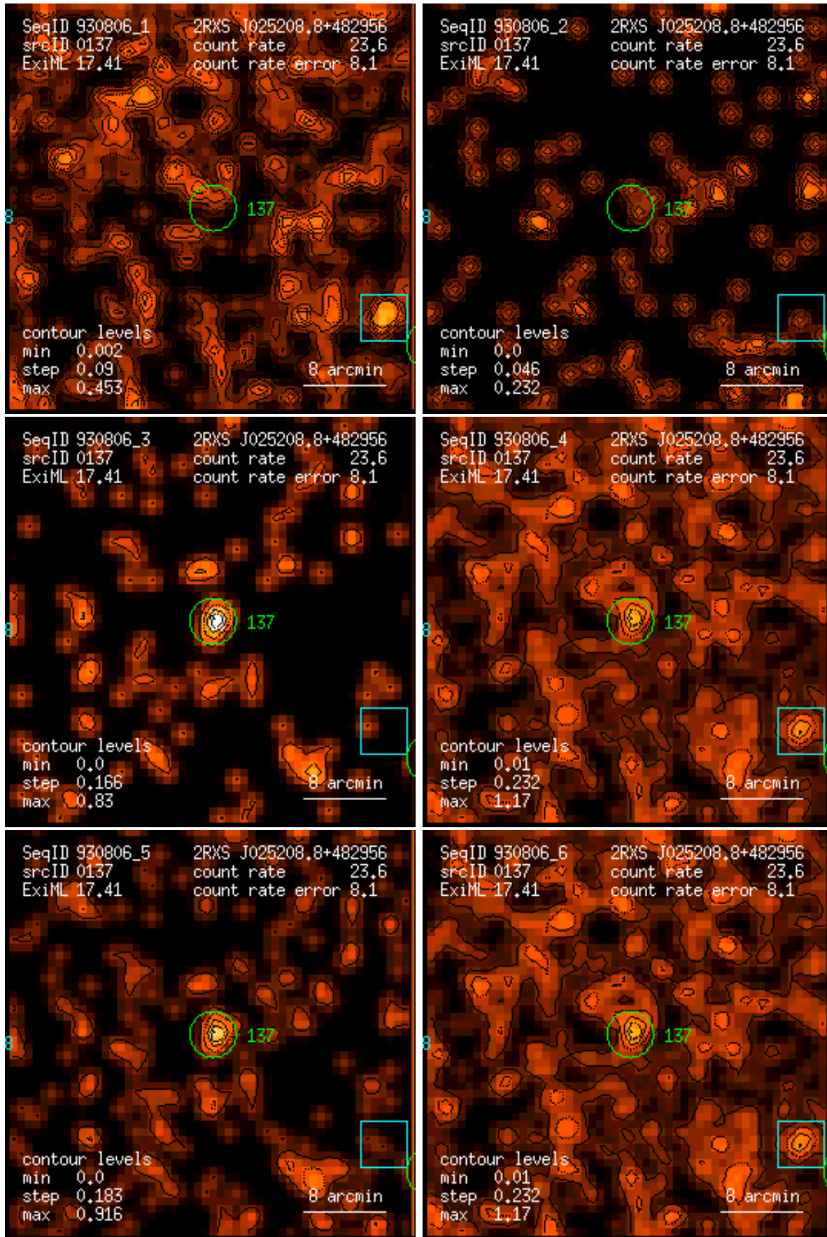
Figure 137: RASS 930806: detection 0137: band rate images, Gaussian filter: (1) PSPC channels 11 – 41, (2) 52 – 90, (3) 91 – 201, (4) 11 – 235, (5) 52 – 201, (6) 11 – 201. Broad band rates in counts/ks. Band rate contour levels in counts/ks/arcmin 2 .
