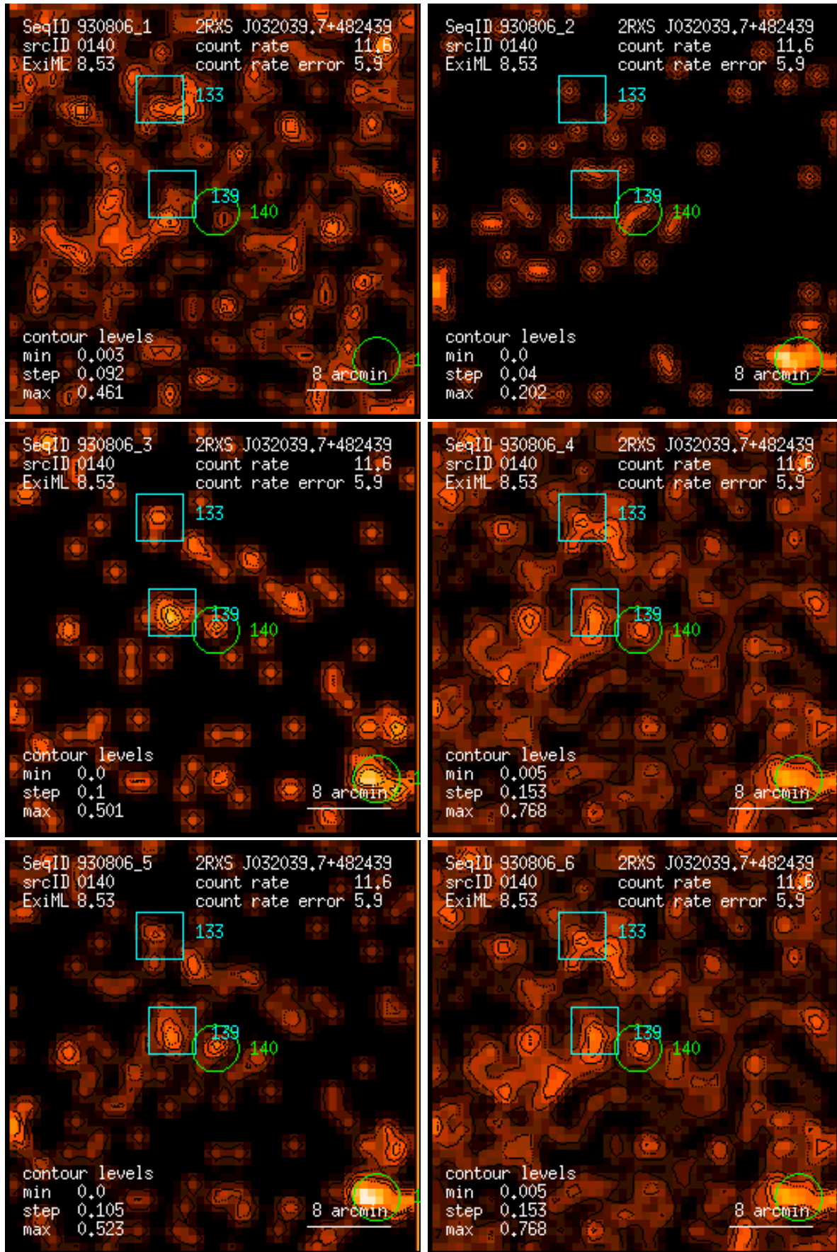
Figure 140: RASS 930806: detection 0140: band rate images, Gaussian filter: (1) PSPC channels 11 – 41, (2) 52 – 90, (3) 91 – 201, (4) 11 – 235, (5) 52 – 201, (6) 11 – 201. Broad band rates in counts/ks. Band rate contour levels in counts/ks/arcmin 2 .
