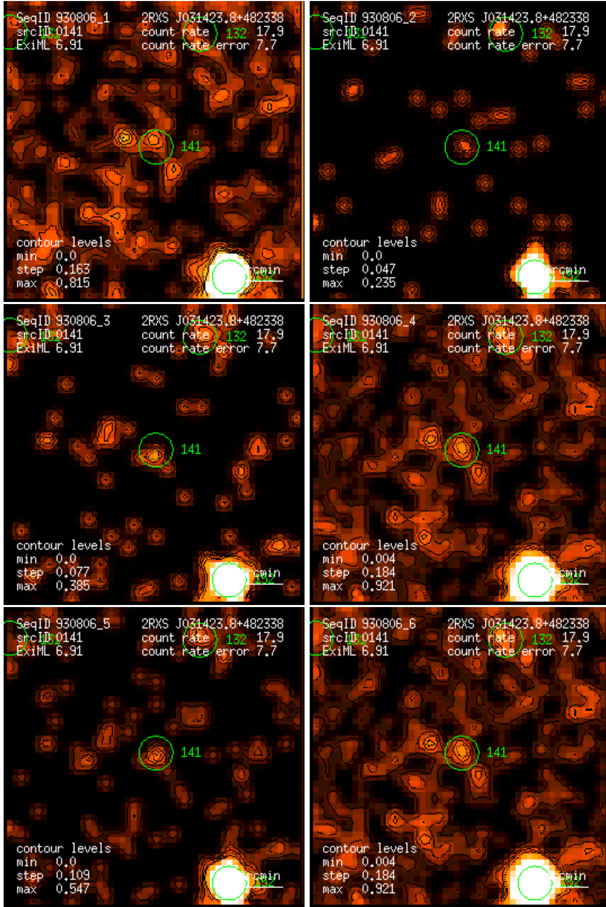
Figure 141: RASS 930806: detection 0141: band rate images, Gaussian filter: (1) PSPC channels 11 – 41, (2) 52 – 90, (3) 91 – 201, (4) 11 – 235, (5) 52 – 201, (6) 11 – 201. Broad band rates in counts/ks. Band rate contour levels in counts/ks/arcmin 2 .
