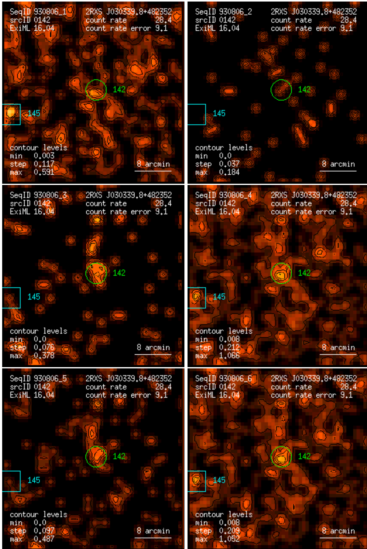
Figure 142: RASS 930806: detection 0142: band rate images, Gaussian filter: (1) PSPC channels 11 – 41, (2) 52 – 90, (3) 91 – 201, (4) 11 – 235, (5) 52 – 201, (6) 11 – 201. Broad band rates in counts/ks. Band rate contour levels in counts/ks/arcmin 2 .
