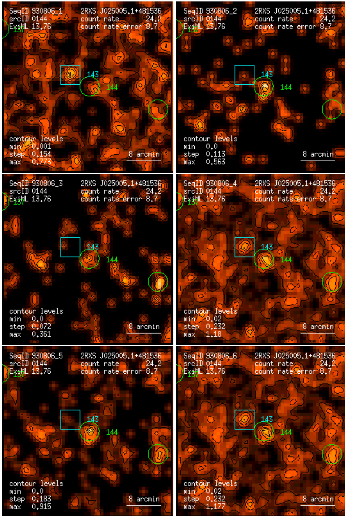
Figure 144: RASS 930806: detection 0144: band rate images, Gaussian filter: (1) PSPC channels 11 – 41, (2) 52 – 90, (3) 91 – 201, (4) 11 – 235, (5) 52 – 201, (6) 11 – 201. Broad band rates in counts/ks. Band rate contour levels in counts/ks/arcmin 2 .
