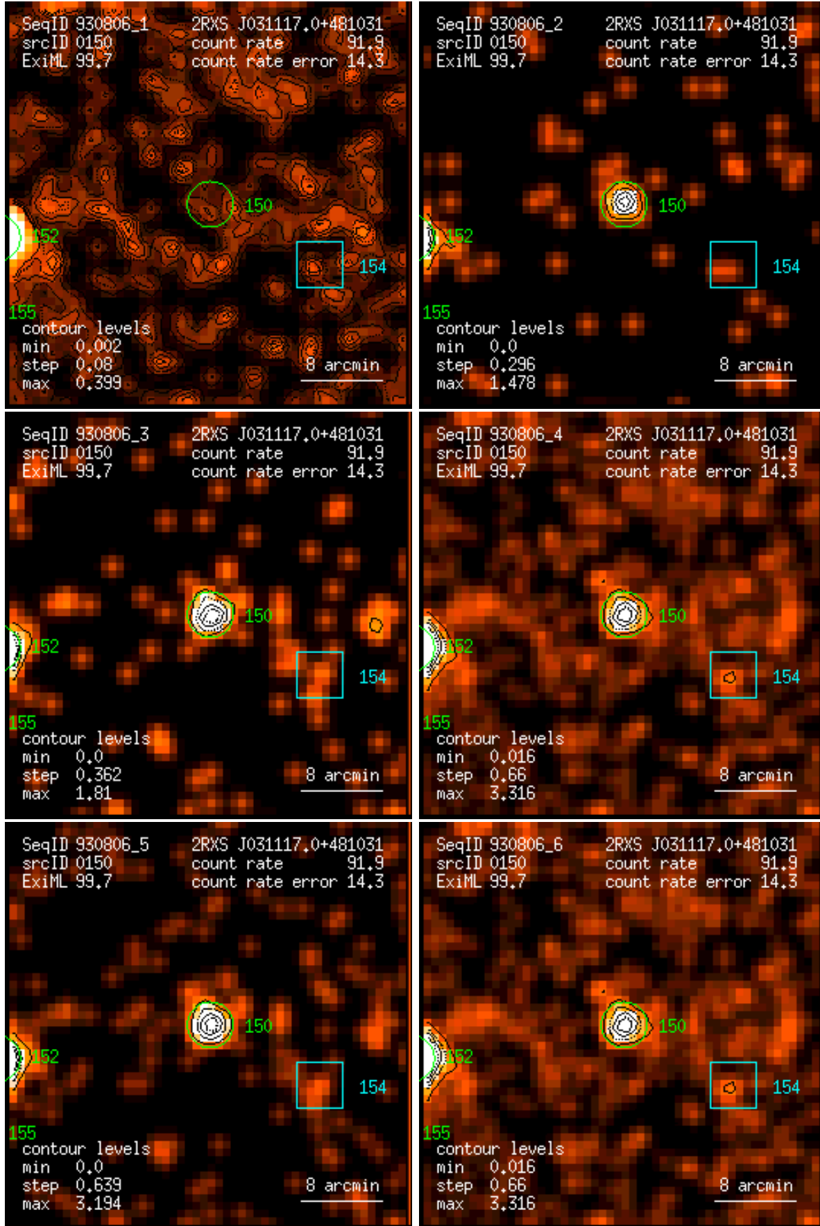
Figure 150: RASS 930806: detection 0150: band rate images, Gaussian filter: (1) PSPC channels 11 – 41, (2) 52 – 90, (3) 91 – 201, (4) 11 – 235, (5) 52 – 201, (6) 11 – 201. Broad band rates in counts/ks. Band rate contour levels in counts/ks/arcmin 2 .
