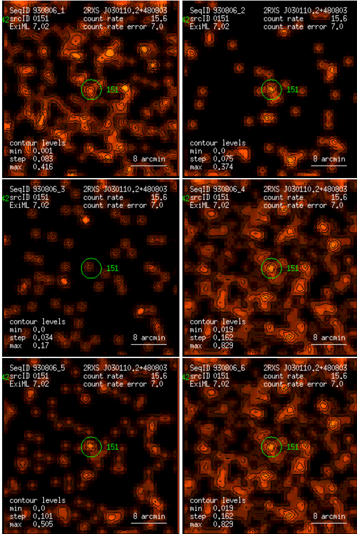
Figure 151: RASS 930806: detection 0151: band rate images, Gaussian filter: (1) PSPC channels 11 – 41, (2) 52 – 90, (3) 91 – 201, (4) 11 – 235, (5) 52 – 201, (6) 11 – 201. Broad band rates in counts/ks. Band rate contour levels in counts/ks/arcmin 2 .
