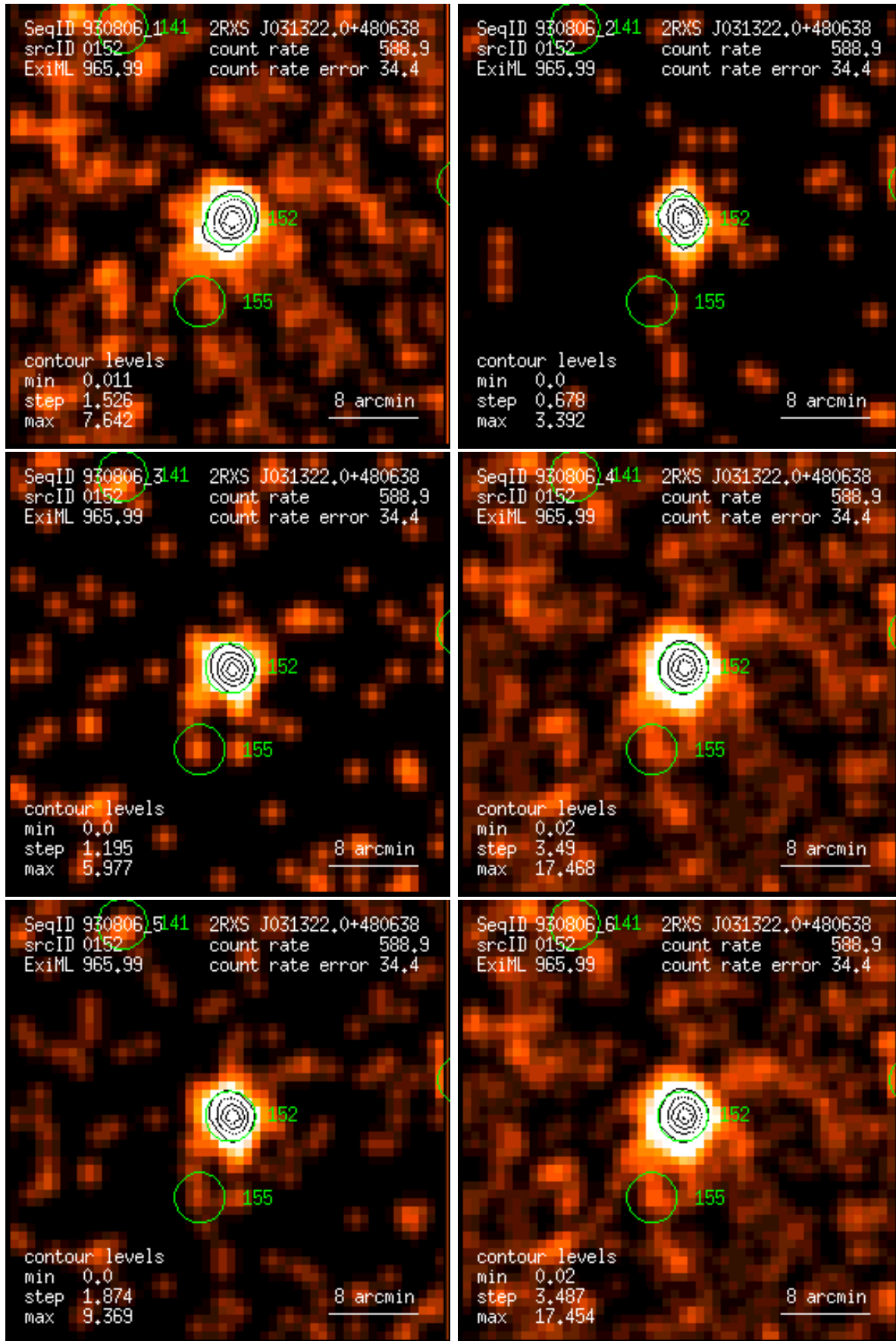
Figure 152: RASS 930806: detection 0152: band rate images, Gaussian filter: (1) PSPC channels 11 – 41, (2) 52 – 90, (3) 91 – 201, (4) 11 – 235, (5) 52 – 201, (6) 11 – 201. Broad band rates in counts/ks. Band rate contour levels in counts/ks/arcmin 2 .
