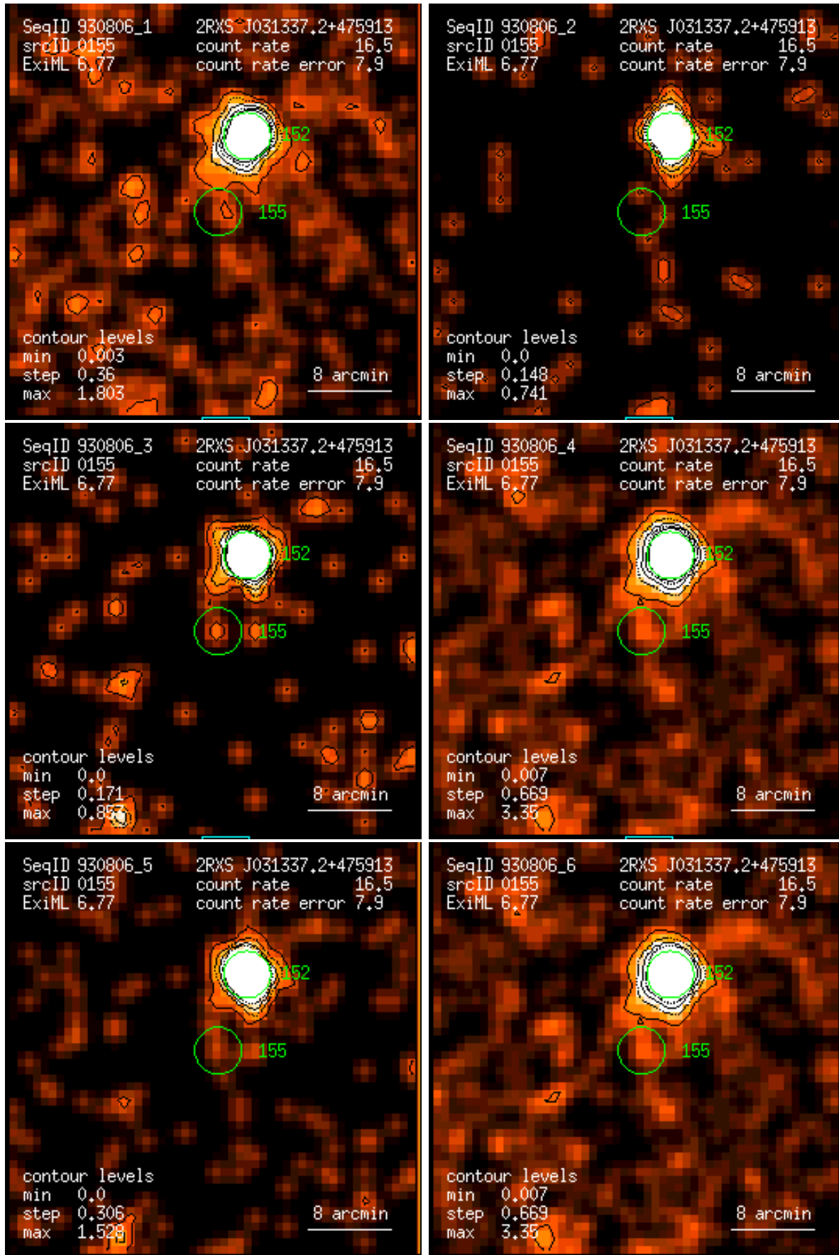
Figure 155: RASS 930806: detection 0155: band rate images, Gaussian filter: (1) PSPC channels 11 – 41, (2) 52 – 90, (3) 91 – 201, (4) 11 – 235, (5) 52 – 201, (6) 11 – 201. Broad band rates in counts/ks. Band rate contour levels in counts/ks/arcmin 2 .
