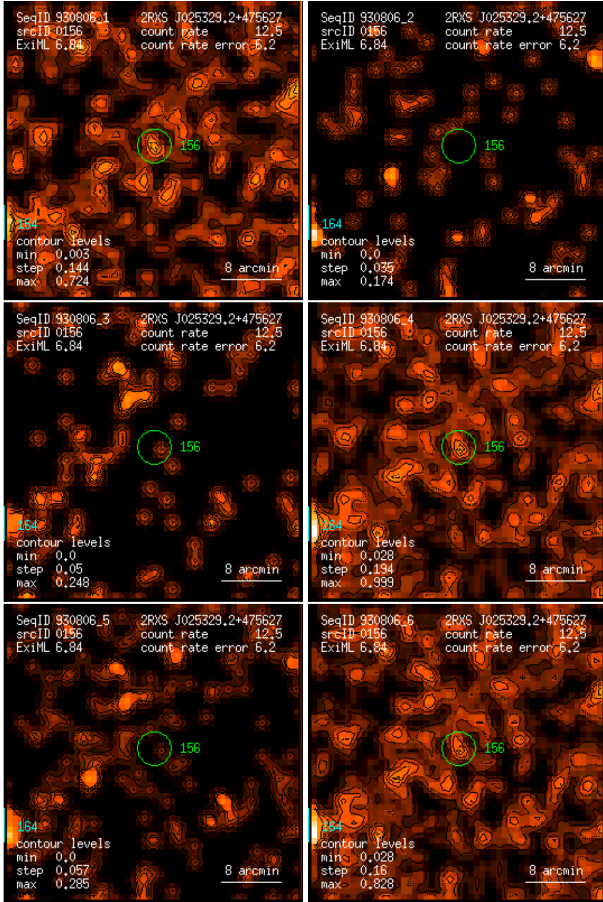
Figure 156: RASS 930806: detection 0156: band rate images, Gaussian filter: (1) PSPC channels 11 – 41, (2) 52 – 90, (3) 91 – 201, (4) 11 – 235, (5) 52 – 201, (6) 11 – 201. Broad band rates in counts/ks. Band rate contour levels in counts/ks/arcmin 2 .
