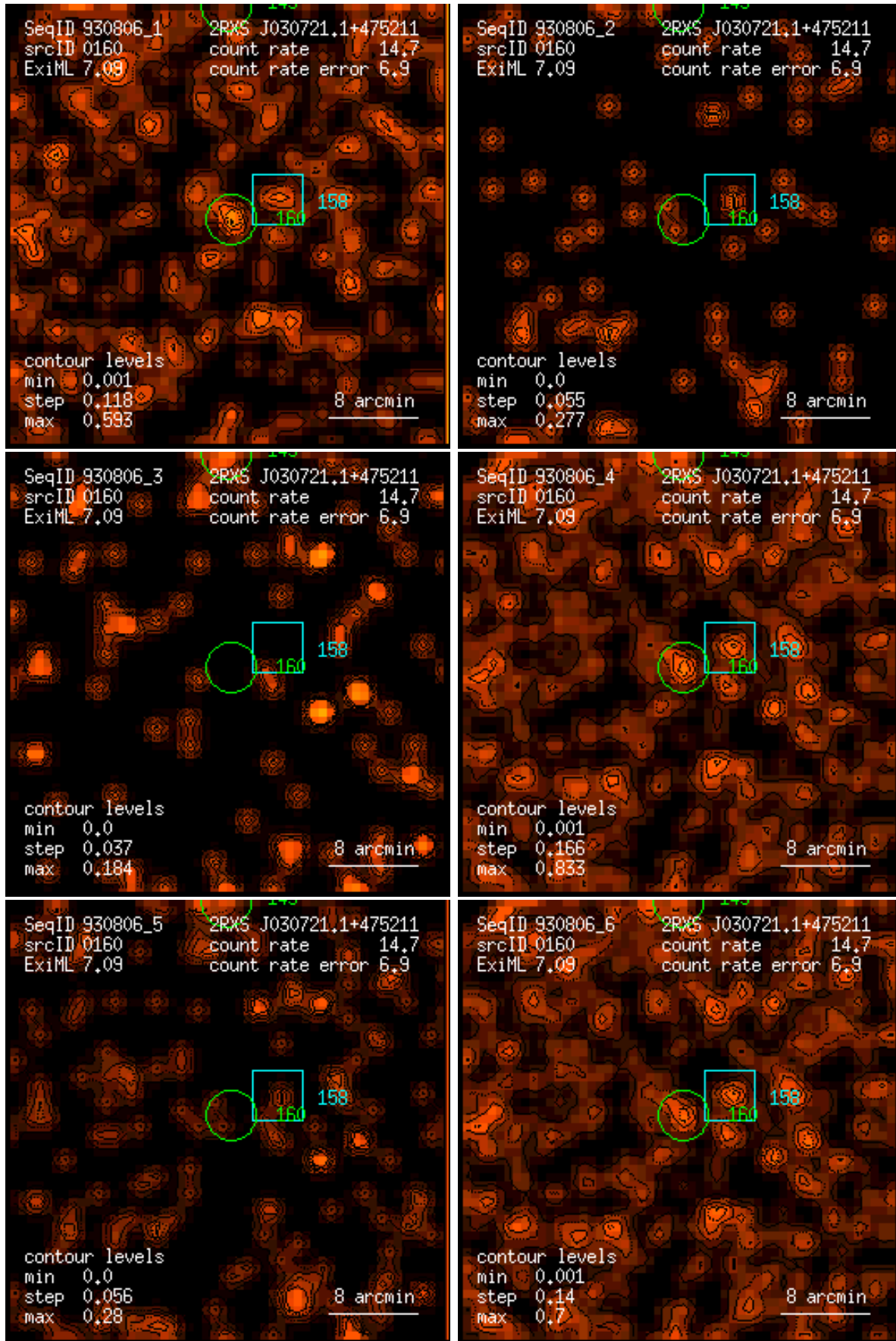
Figure 160: RASS 930806: detection 0160: band rate images, Gaussian filter: (1) PSPC channels 11 – 41, (2) 52 – 90, (3) 91 – 201, (4) 11 – 235, (5) 52 – 201, (6) 11 – 201. Broad band rates in counts/ks. Band rate contour levels in counts/ks/arcmin 2 .
