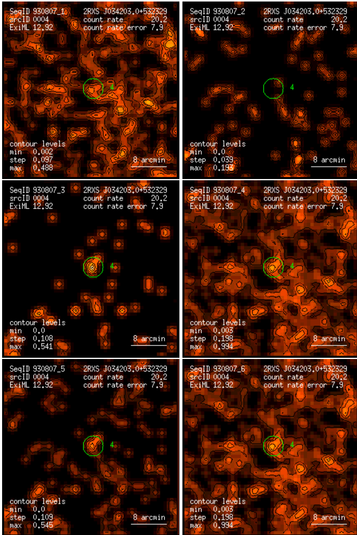
Figure 4: RASS 930807: detection 0004: band rate images, Gaussian filter: (1) PSPC channels 11 – 41, (2) 52 – 90, (3) 91 – 201, (4) 11 – 235, (5) 52 – 201, (6) 11 – 201. Broad band rates in counts/ks. Band rate contour levels in counts/ks/arcmin 2 .
