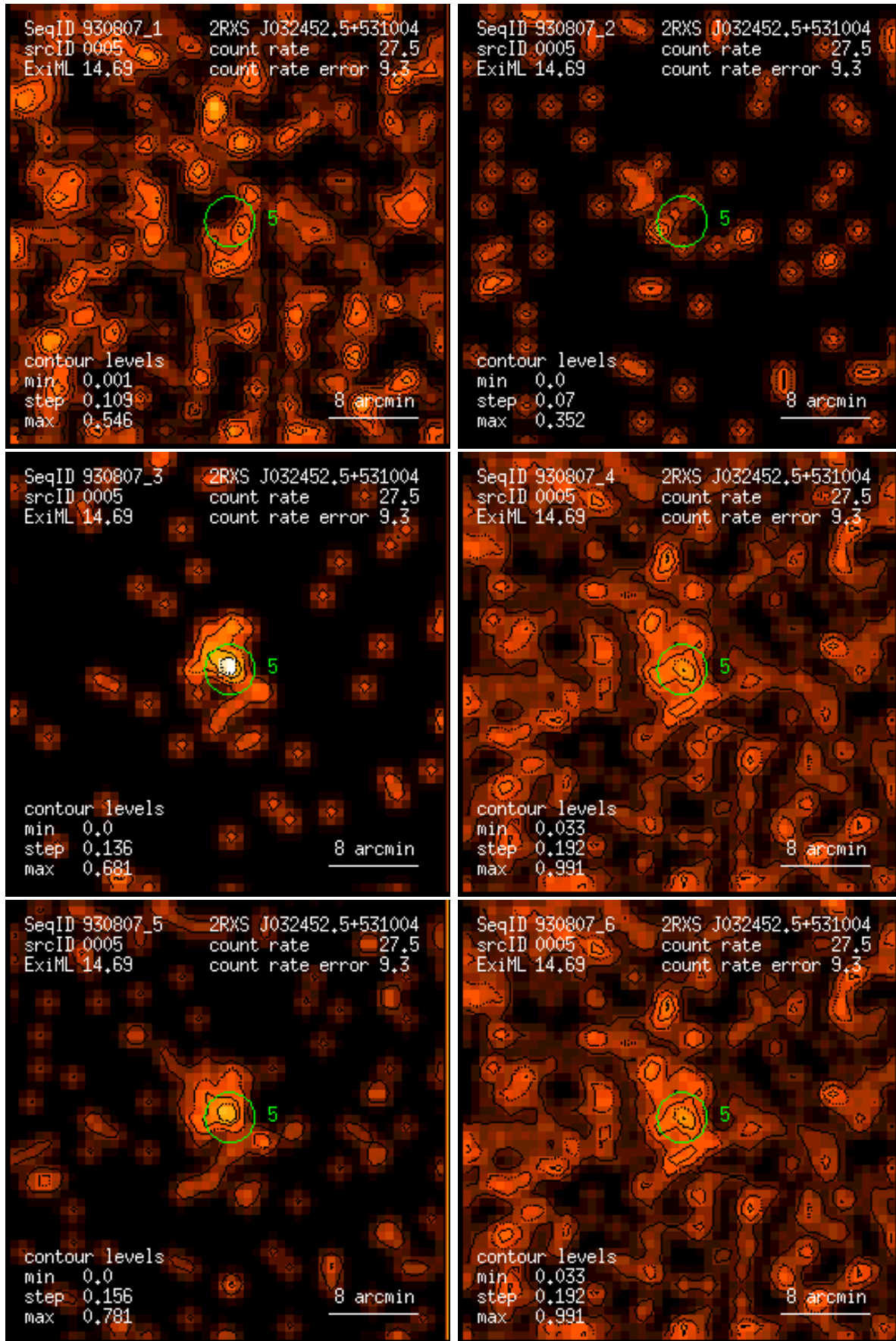
Figure 5: RASS 930807: detection 0005: band rate images, Gaussian filter: (1) PSPC channels 11 – 41, (2) 52 – 90, (3) 91 – 201, (4) 11 – 235, (5) 52 – 201, (6) 11 – 201. Broad band rates in counts/ks. Band rate contour levels in counts/ks/arcmin 2 .
