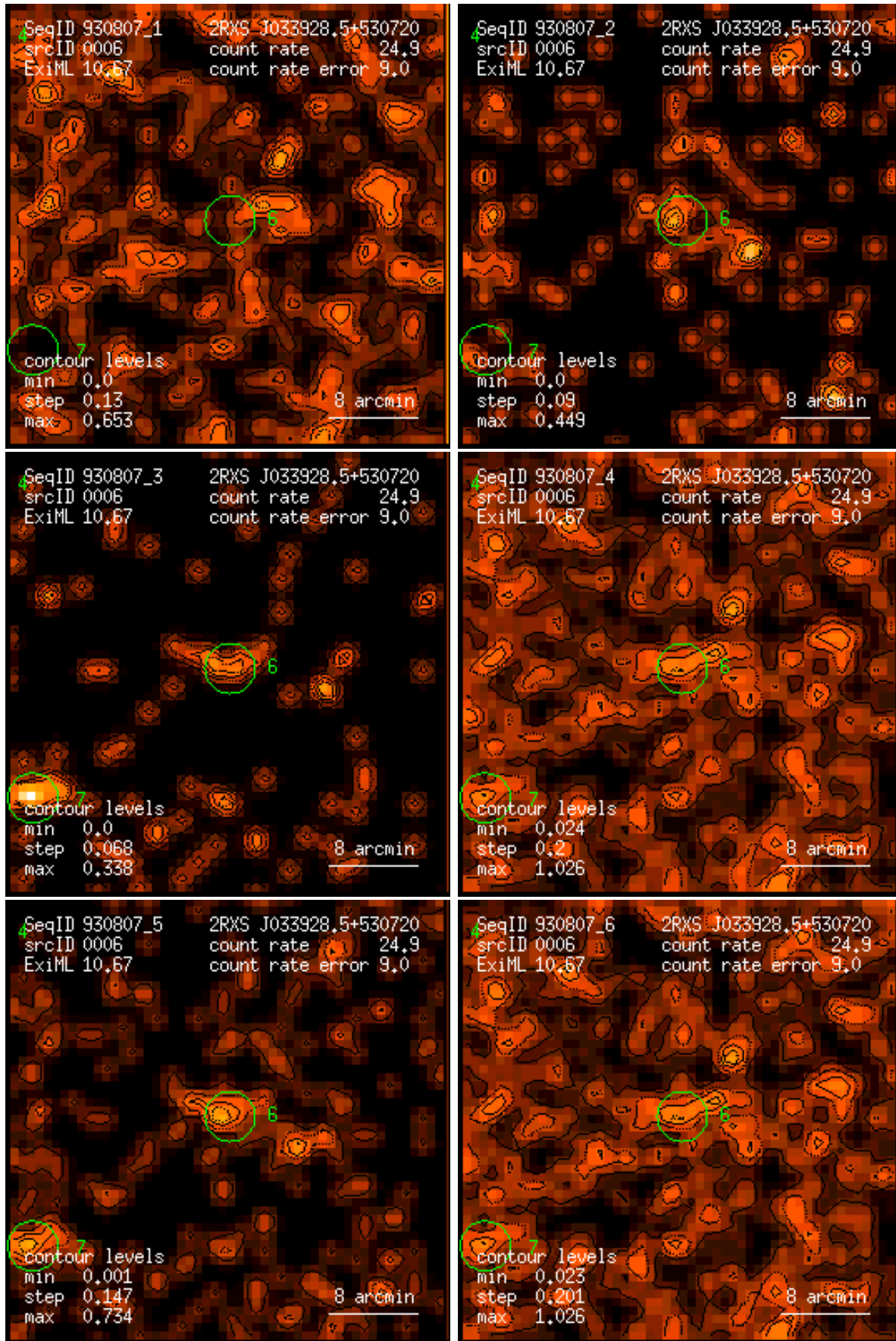
Figure 6: RASS 930807: detection 0006: band rate images, Gaussian filter: (1) PSPC channels 11 – 41, (2) 52 – 90, (3) 91 – 201, (4) 11 – 235, (5) 52 – 201, (6) 11 – 201. Broad band rates in counts/ks. Band rate contour levels in counts/ks/arcmin 2 .
