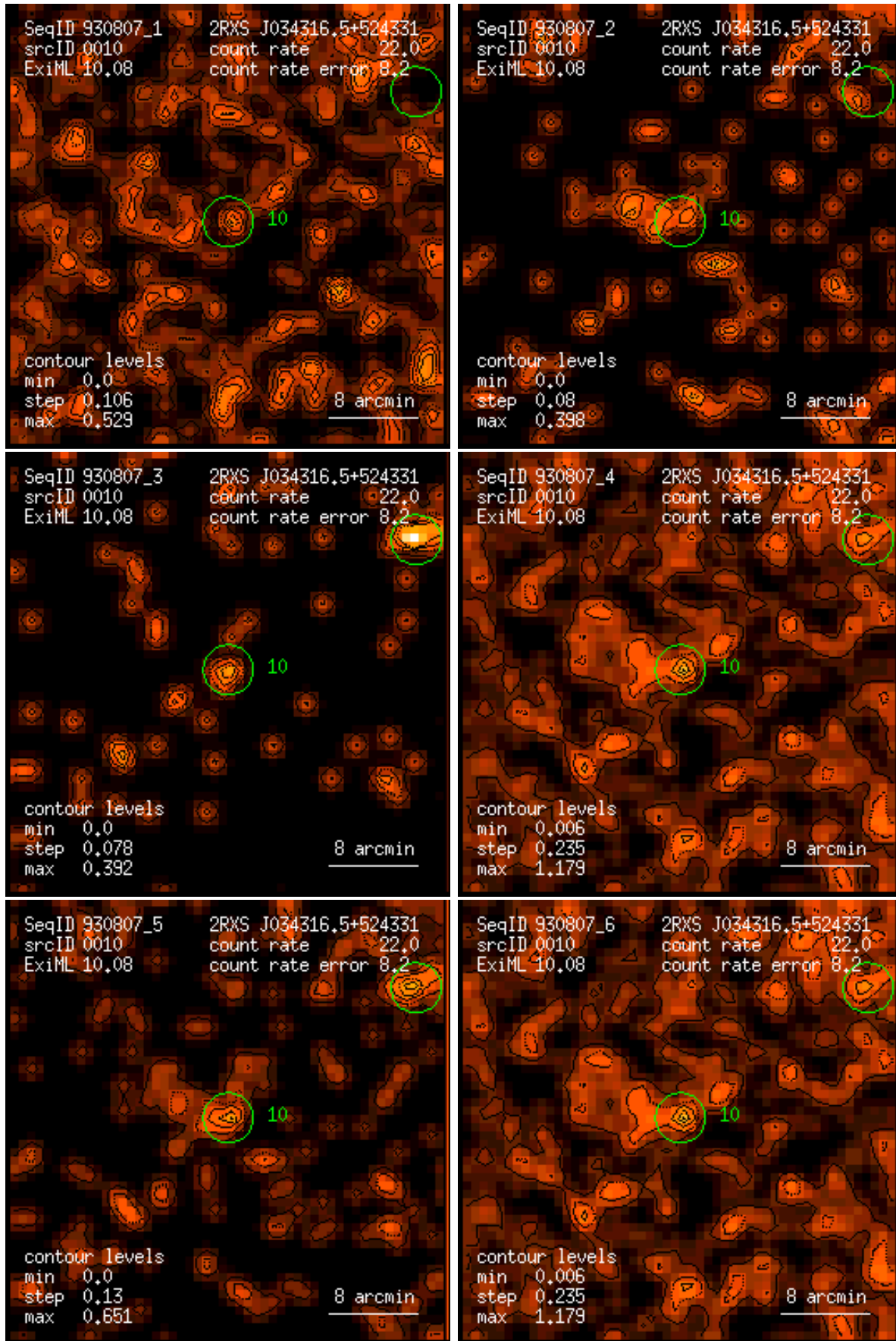
Figure 10: RASS 930807: detection 0010: band rate images, Gaussian filter: (1) PSPC channels 11 – 41, (2) 52 – 90, (3) 91 – 201, (4) 11 – 235, (5) 52 – 201, (6) 11 – 201. Broad band rates in counts/ks. Band rate contour levels in counts/ks/arcmin 2 .
