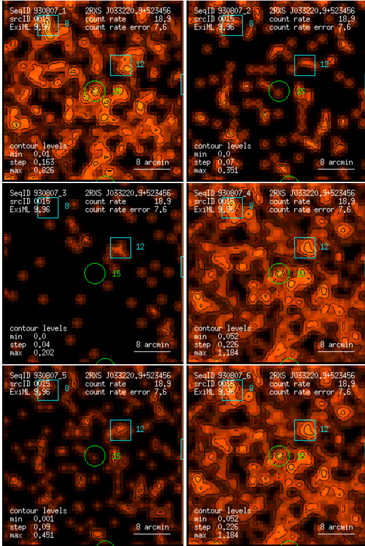
Figure 15: RASS 930807: detection 0015: band rate images, Gaussian filter: (1) PSPC channels 11 – 41, (2) 52 – 90, (3) 91 – 201, (4) 11 – 235, (5) 52 – 201, (6) 11 – 201. Broad band rates in counts/ks. Band rate contour levels in counts/ks/arcmin 2 .
