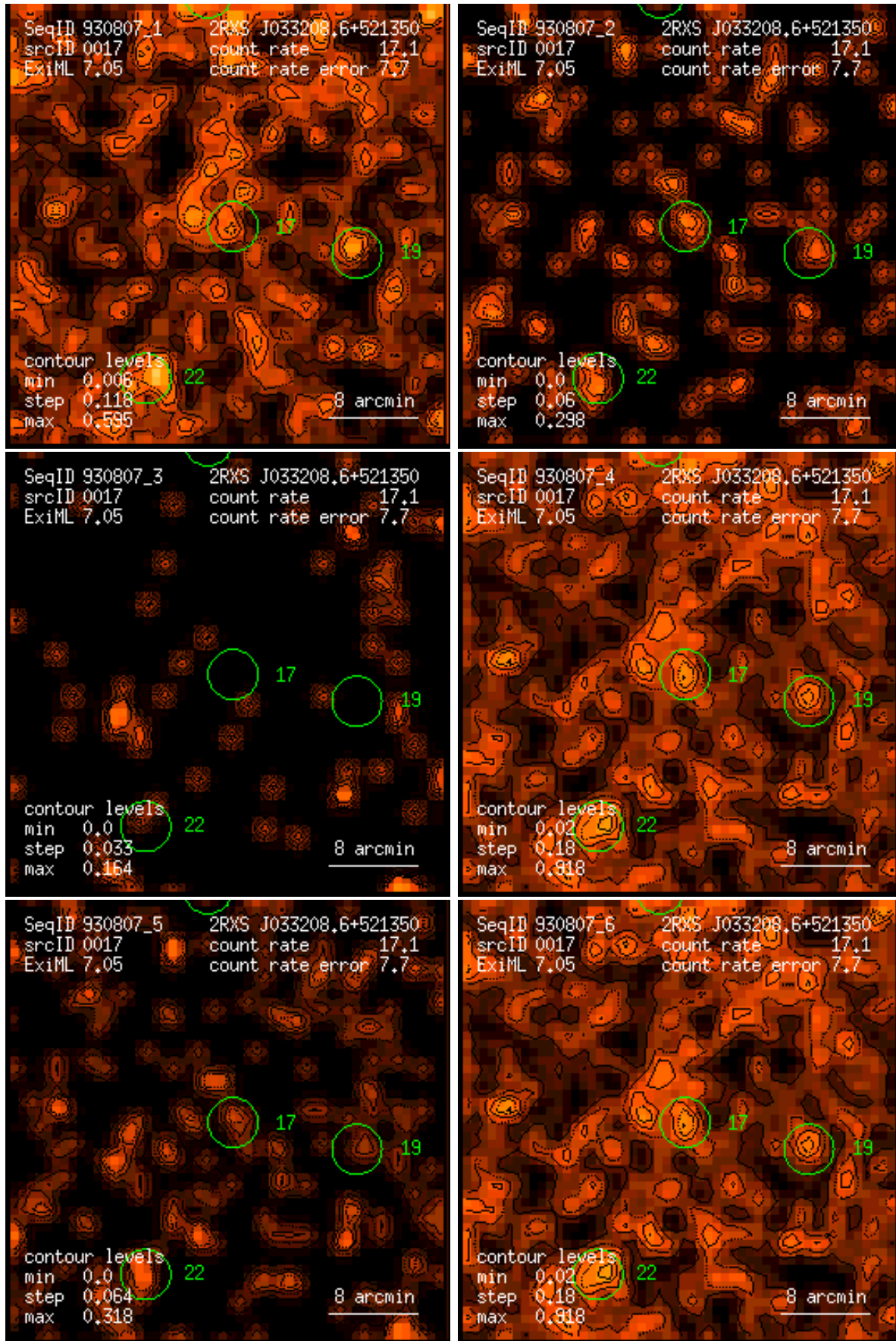
Figure 17: RASS 930807: detection 0017: band rate images, Gaussian filter: (1) PSPC channels 11 – 41, (2) 52 – 90, (3) 91 – 201, (4) 11 – 235, (5) 52 – 201, (6) 11 – 201. Broad band rates in counts/ks. Band rate contour levels in counts/ks/arcmin 2 .
