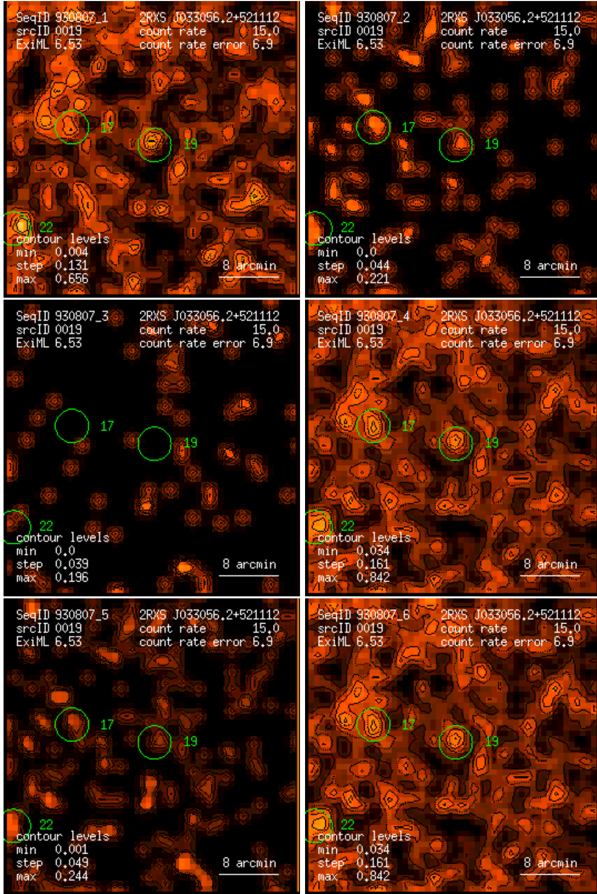
Figure 19: RASS 930807: detection 0019: band rate images, Gaussian filter: (1) PSPC channels 11 – 41, (2) 52 – 90, (3) 91 – 201, (4) 11 – 235, (5) 52 – 201, (6) 11 – 201. Broad band rates in counts/ks. Band rate contour levels in counts/ks/arcmin 2 .
