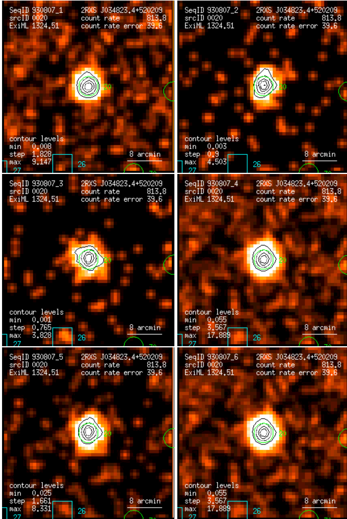
Figure 20: RASS 930807: detection 0020: band rate images, Gaussian filter: (1) PSPC channels 11 – 41, (2) 52 – 90, (3) 91 – 201, (4) 11 – 235, (5) 52 – 201, (6) 11 – 201. Broad band rates in counts/ks. Band rate contour levels in counts/ks/arcmin 2 .
