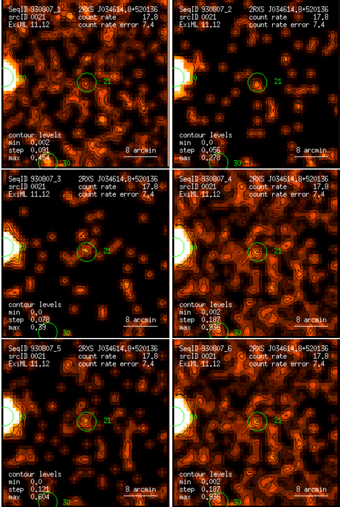
Figure 21: RASS 930807: detection 0021: band rate images, Gaussian filter: (1) PSPC channels 11 – 41, (2) 52 – 90, (3) 91 – 201, (4) 11 – 235, (5) 52 – 201, (6) 11 – 201. Broad band rates in counts/ks. Band rate contour levels in counts/ks/arcmin 2 .
