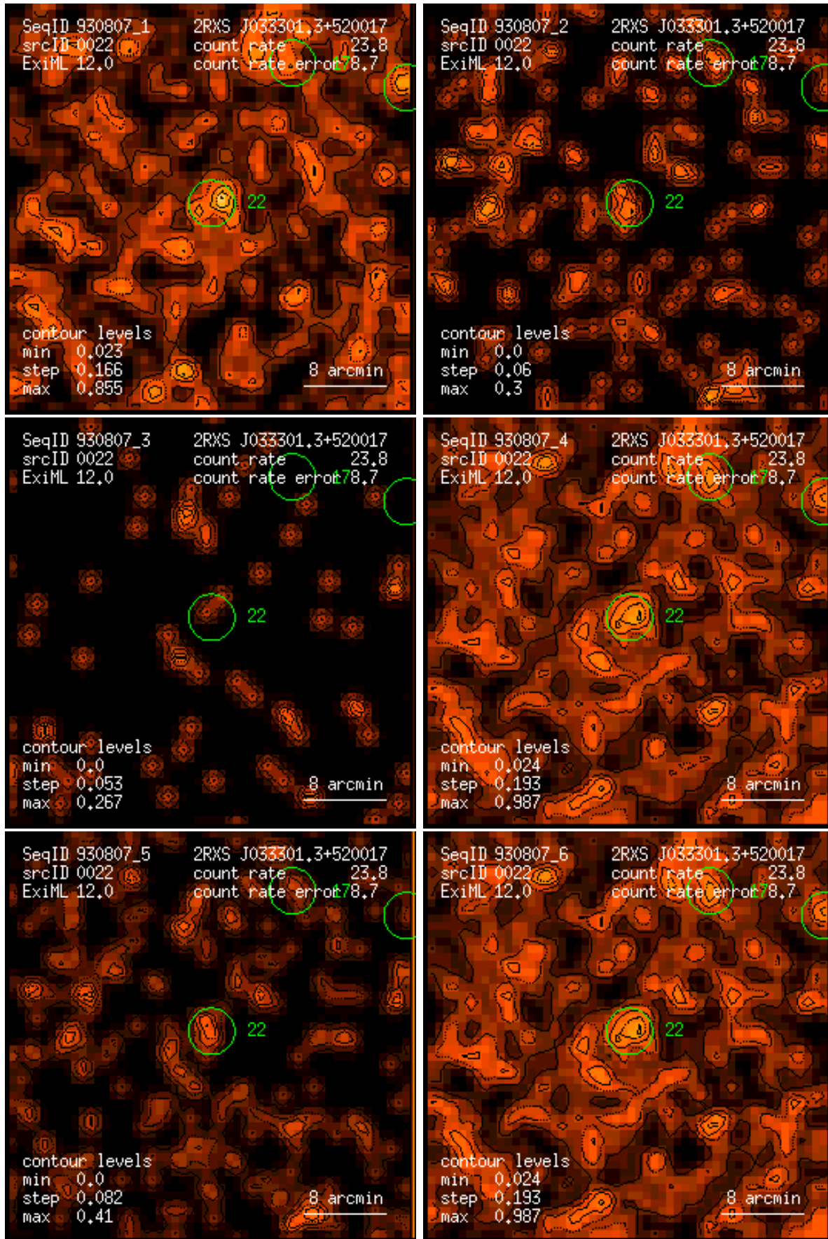
Figure 22: RASS 930807: detection 0022: band rate images, Gaussian filter: (1) PSPC channels 11 – 41, (2) 52 – 90, (3) 91 – 201, (4) 11 – 235, (5) 52 – 201, (6) 11 – 201. Broad band rates in counts/ks. Band rate contour levels in counts/ks/arcmin 2 .
