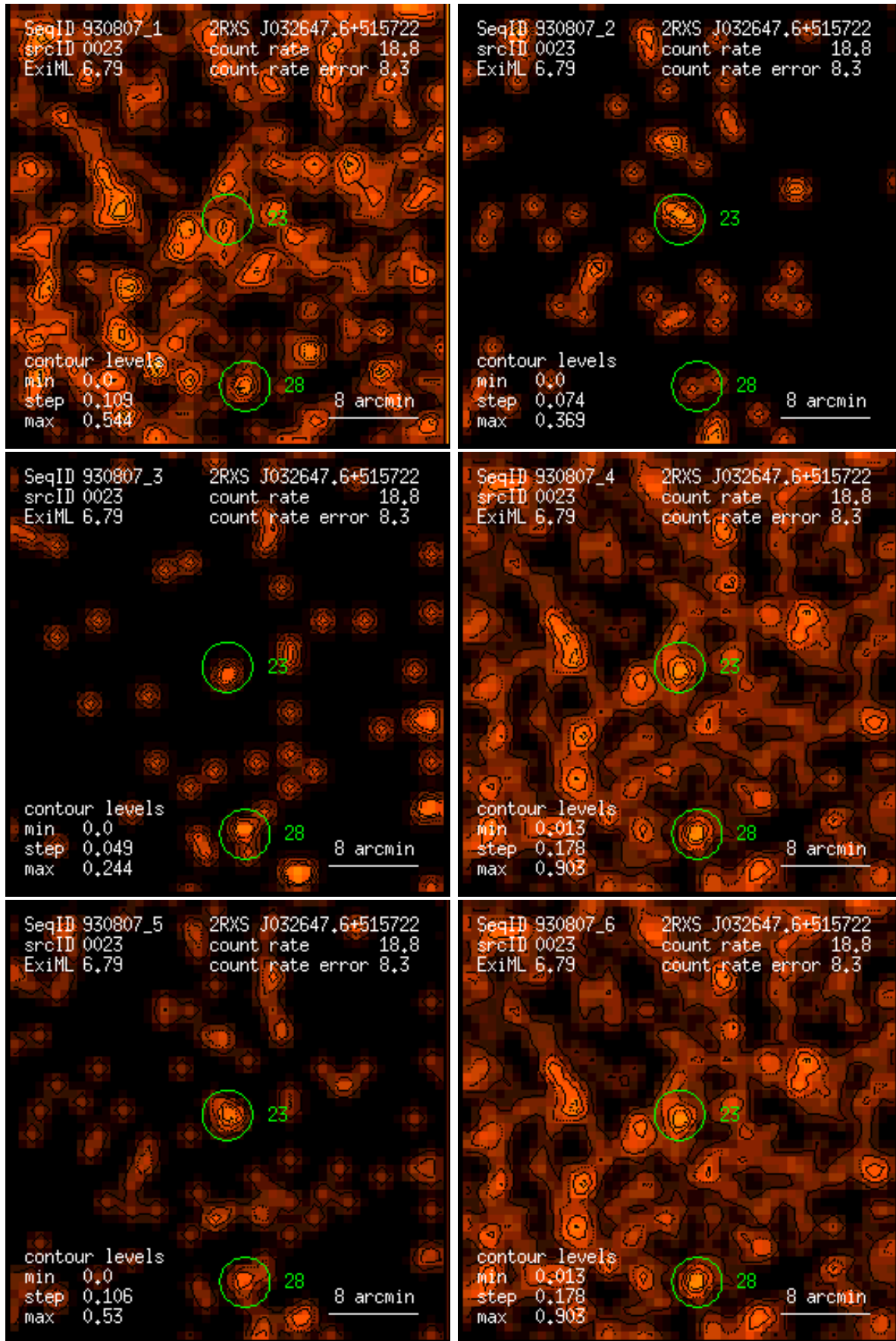
Figure 23: RASS 930807: detection 0023: band rate images, Gaussian filter: (1) PSPC channels 11 – 41, (2) 52 – 90, (3) 91 – 201, (4) 11 – 235, (5) 52 – 201, (6) 11 – 201. Broad band rates in counts/ks. Band rate contour levels in counts/ks/arcmin 2 .
