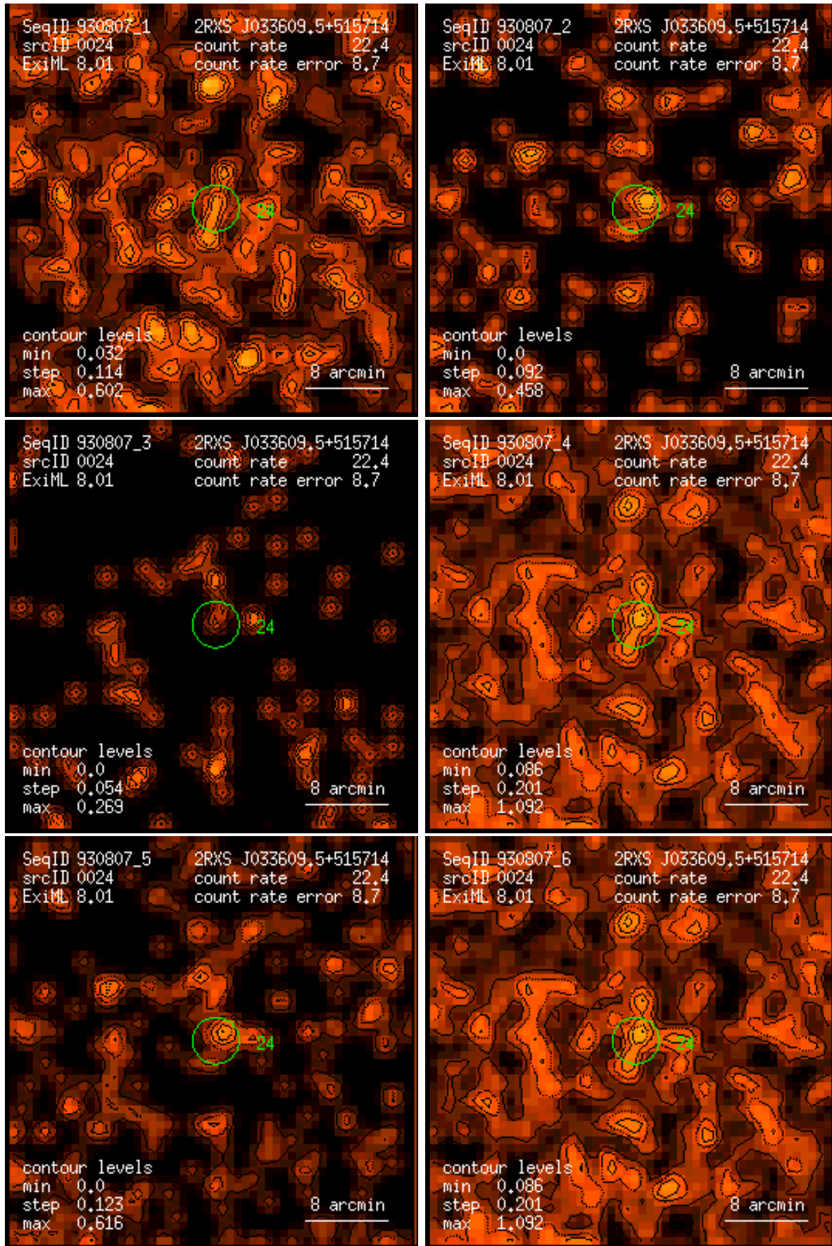
Figure 24: RASS 930807: detection 0024: band rate images, Gaussian filter: (1) PSPC channels 11 – 41, (2) 52 – 90, (3) 91 – 201, (4) 11 – 235, (5) 52 – 201, (6) 11 – 201. Broad band rates in counts/ks. Band rate contour levels in counts/ks/arcmin 2 .
