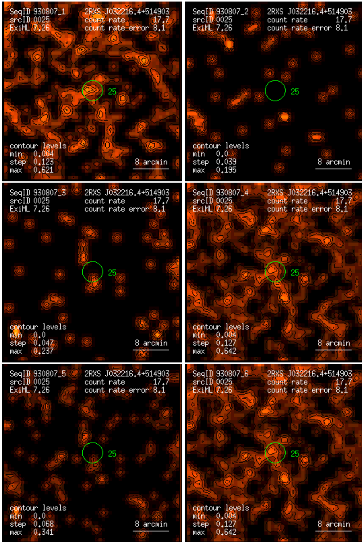
Figure 25: RASS 930807: detection 0025: band rate images, Gaussian filter: (1) PSPC channels 11 – 41, (2) 52 – 90, (3) 91 – 201, (4) 11 – 235, (5) 52 – 201, (6) 11 – 201. Broad band rates in counts/ks. Band rate contour levels in counts/ks/arcmin 2 .
