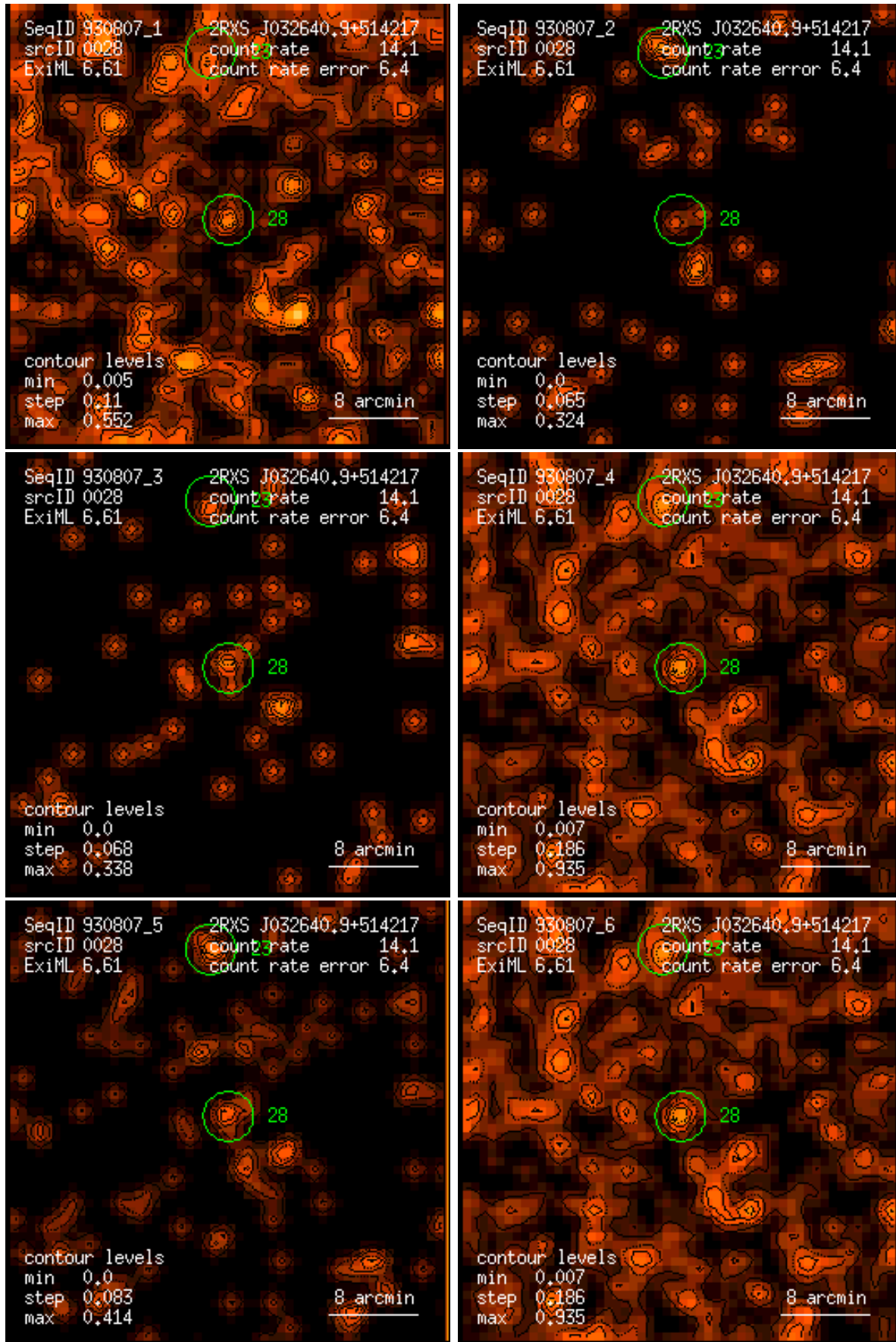
Figure 28: RASS 930807: detection 0028: band rate images, Gaussian filter: (1) PSPC channels 11 – 41, (2) 52 – 90, (3) 91 – 201, (4) 11 – 235, (5) 52 – 201, (6) 11 – 201. Broad band rates in counts/ks. Band rate contour levels in counts/ks/arcmin 2 .
