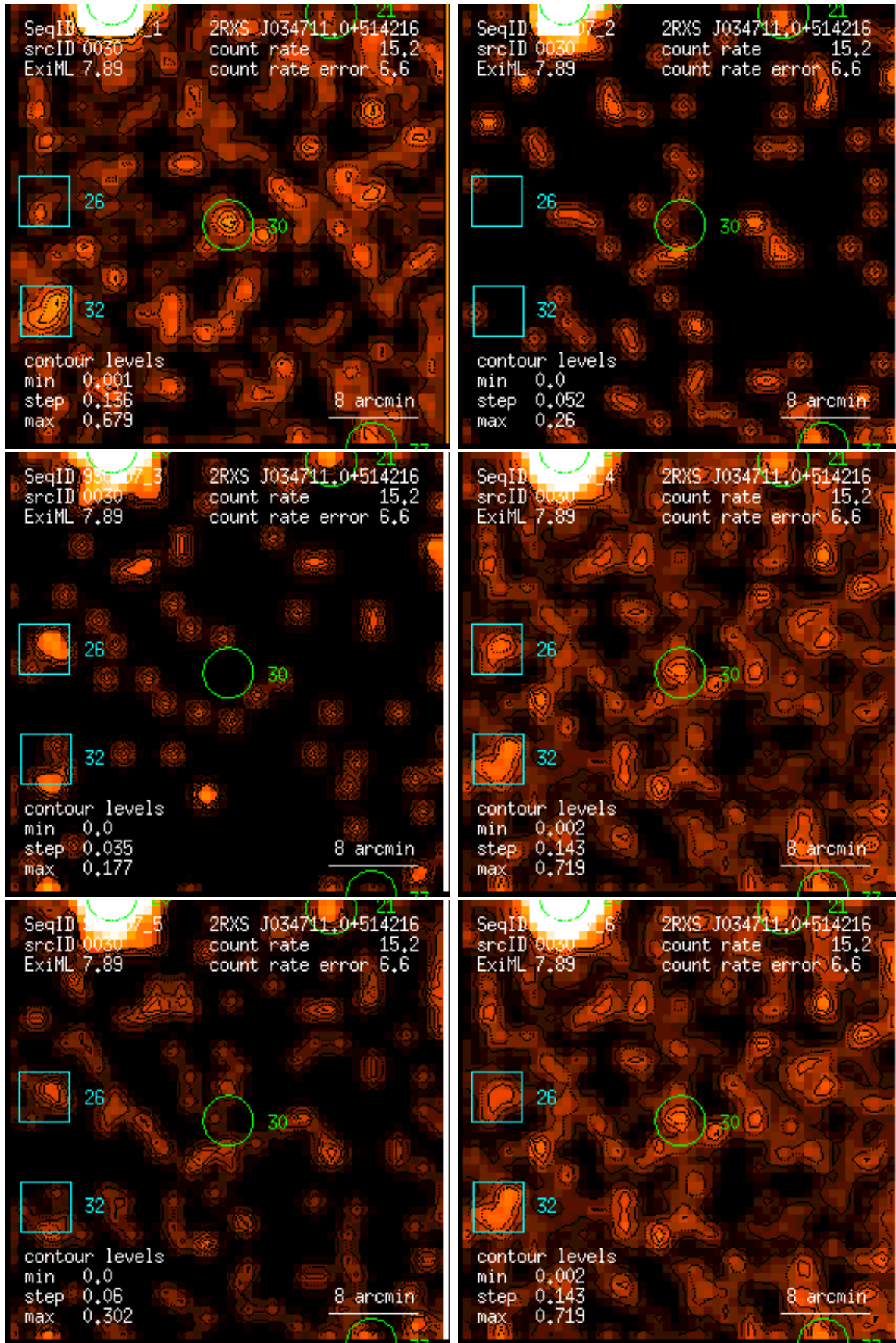
Figure 30: RASS 930807: detection 0030: band rate images, Gaussian filter: (1) PSPC channels 11 – 41, (2) 52 – 90, (3) 91 – 201, (4) 11 – 235, (5) 52 – 201, (6) 11 – 201. Broad band rates in counts/ks. Band rate contour levels in counts/ks/arcmin 2 .
