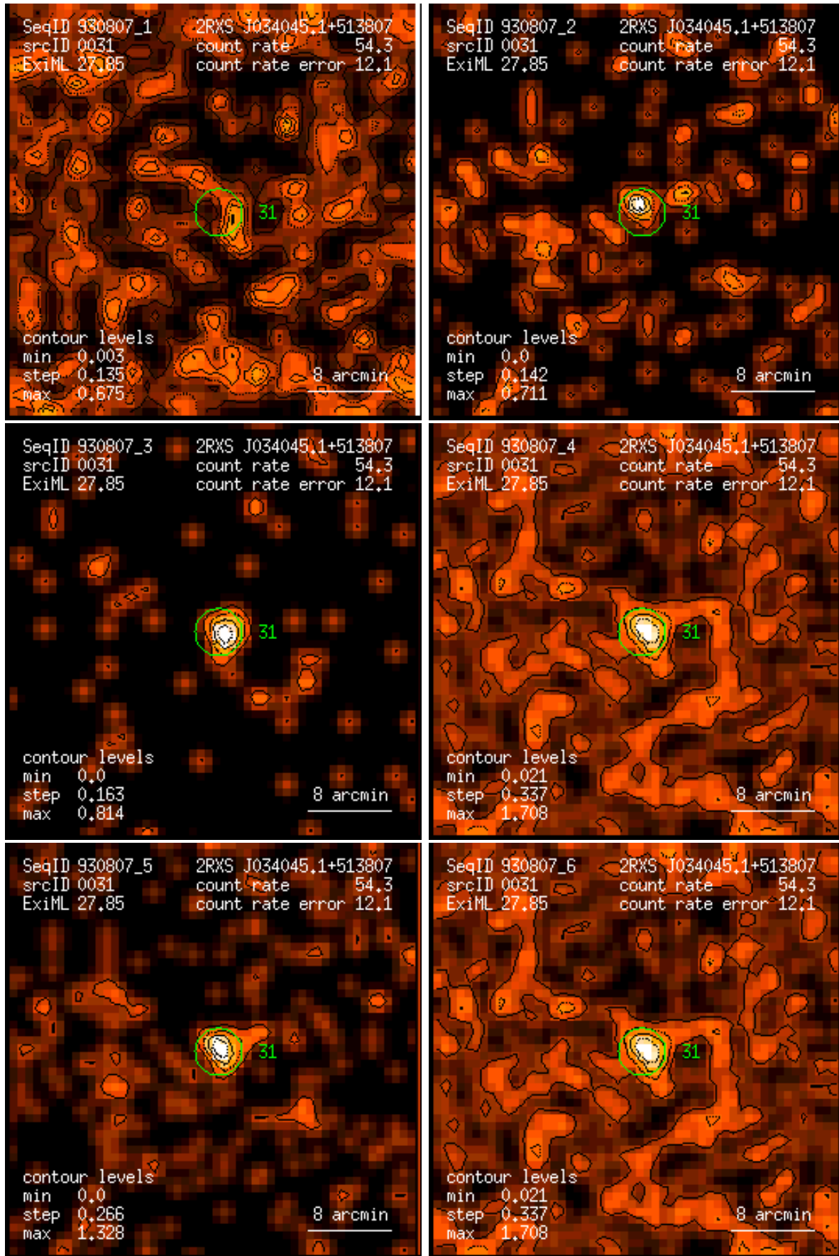
Figure 31: RASS 930807: detection 0031: band rate images, Gaussian filter: (1) PSPC channels 11 – 41, (2) 52 – 90, (3) 91 – 201, (4) 11 – 235, (5) 52 – 201, (6) 11 – 201. Broad band rates in counts/ks. Band rate contour levels in counts/ks/arcmin 2 .
