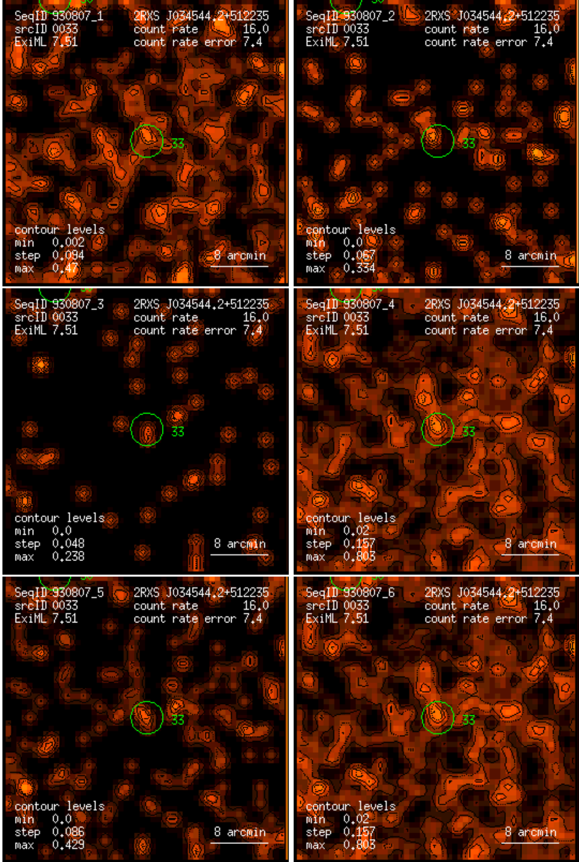
Figure 33: RASS 930807: detection 0033: band rate images, Gaussian filter: (1) PSPC channels 11 – 41, (2) 52 – 90, (3) 91 – 201, (4) 11 – 235, (5) 52 – 201, (6) 11 – 201. Broad band rates in counts/ks. Band rate contour levels in counts/ks/arcmin 2 .
