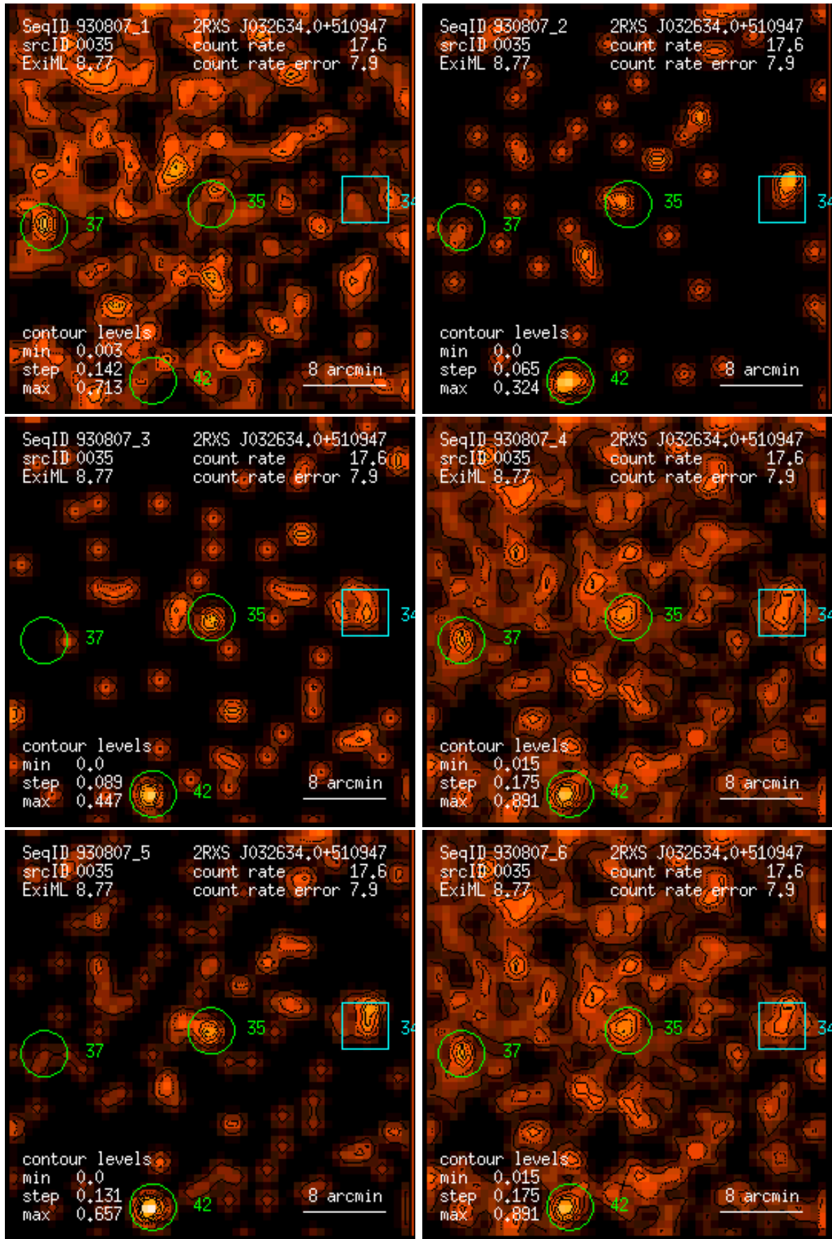
Figure 35: RASS 930807: detection 0035: band rate images, Gaussian filter: (1) PSPC channels 11 – 41, (2) 52 – 90, (3) 91 – 201, (4) 11 – 235, (5) 52 – 201, (6) 11 – 201. Broad band rates in counts/ks. Band rate contour levels in counts/ks/arcmin 2 .
