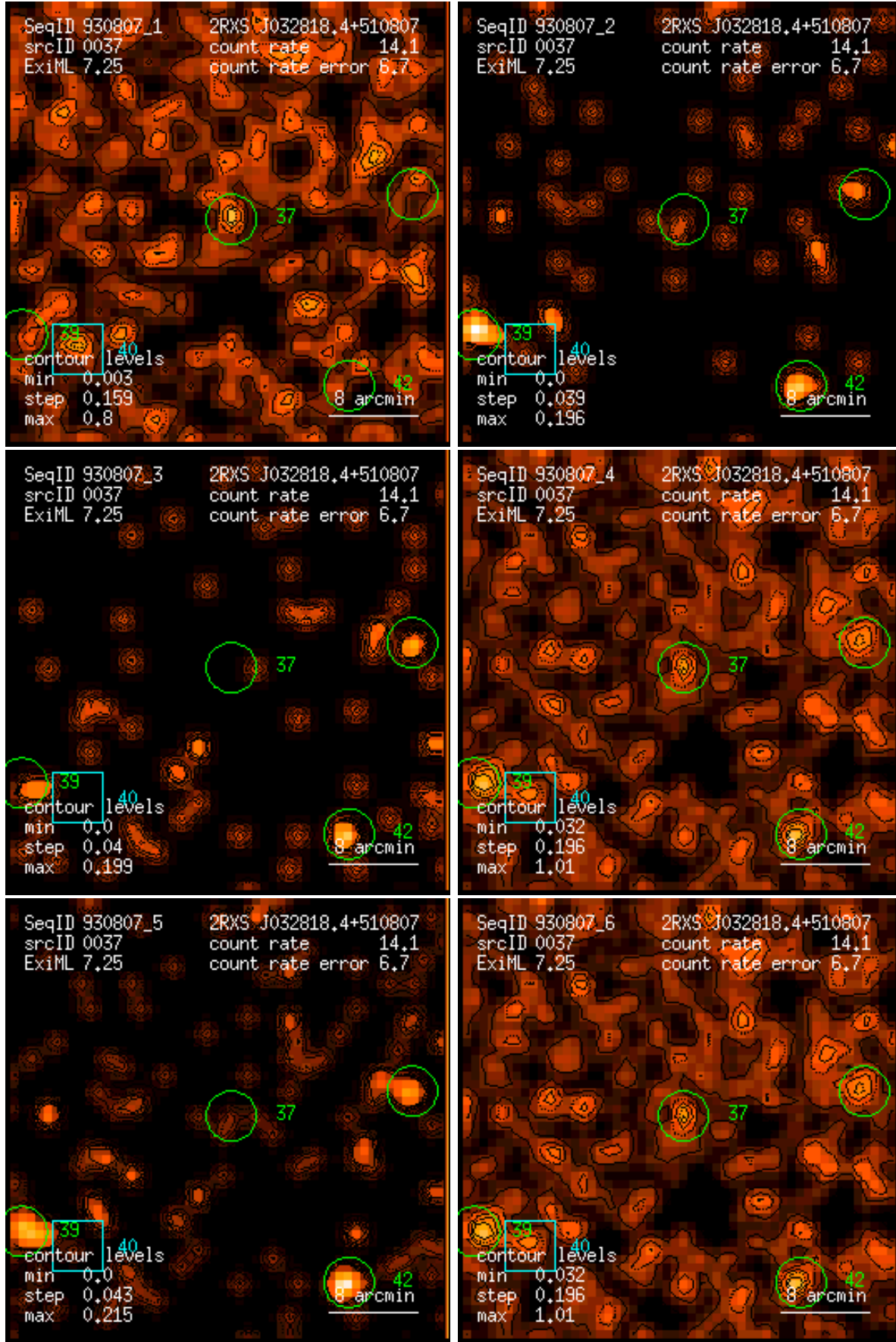
Figure 37: RASS 930807: detection 0037: band rate images, Gaussian filter: (1) PSPC channels 11 – 41, (2) 52 – 90, (3) 91 – 201, (4) 11 – 235, (5) 52 – 201, (6) 11 – 201. Broad band rates in counts/ks. Band rate contour levels in counts/ks/arcmin 2 .
